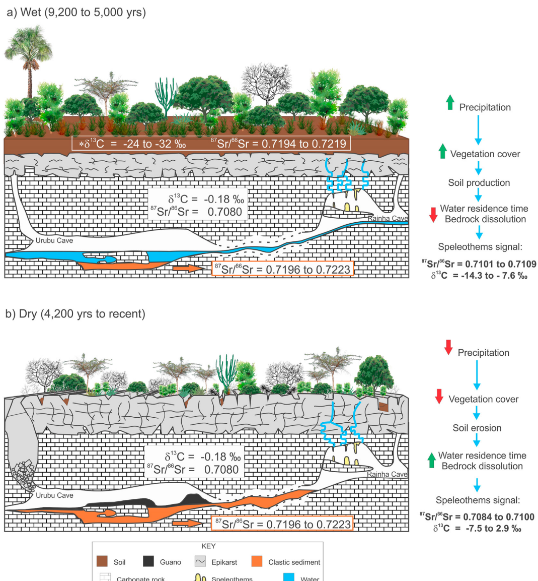
Fig. 6. Conceptual model for the environmental changes in the Rainha-Urubu cave system based on isotopic proxies: a) wet conditions observed from 9,200 to 5,000 yrs BP and b) dry conditions observed from 4,200 yrs BP to the present.
