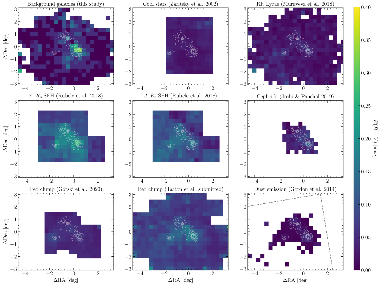
Figure 6. 20 \times 20 arcmin 2 resolution reddening maps covering the SMC. Each panel refers to a different literature source. The contours in all panels represent the IRAS 100 \mu m dust emission. The dashed line in the lower right panel represents the footprint of the HERITAGE observations.
