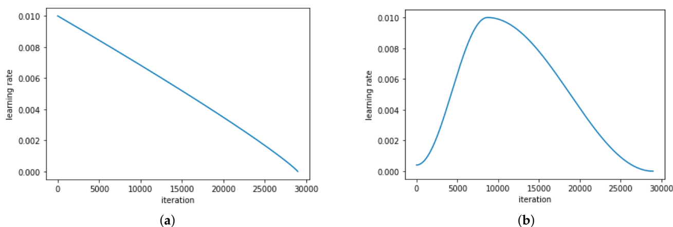
Figure 9. The two learning rate schedulers (LRS): (a) Poly and (b) OneCycle.
