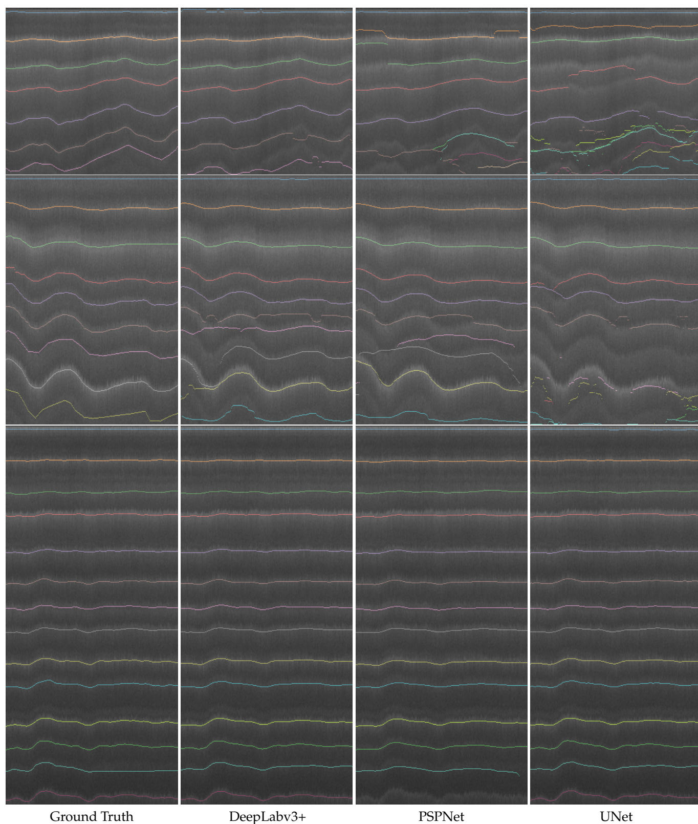
Figure 12. Radar images overlaid with Ground Truth layers ( first column ) and layers predicted from the three FCNs: DeepLabv3+ ( second column ), PSPNet ( third column ), and UNet ( fourth column ). The results shown are from each network's best output in terms of mean IoU (Table 3). More examples are in Figure 11.
