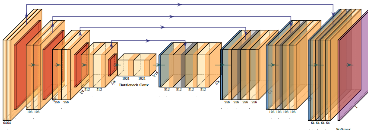
Figure 6. UNet [13] architecture. Green arrows depict forward connections, and purple arrows depict skip connections. ‘ T/x ’ denotes a downsampled, spatially reduced, input image ‘ T ’, while 64, 128, 256, and 512 denote the channel numbers at each layer.
