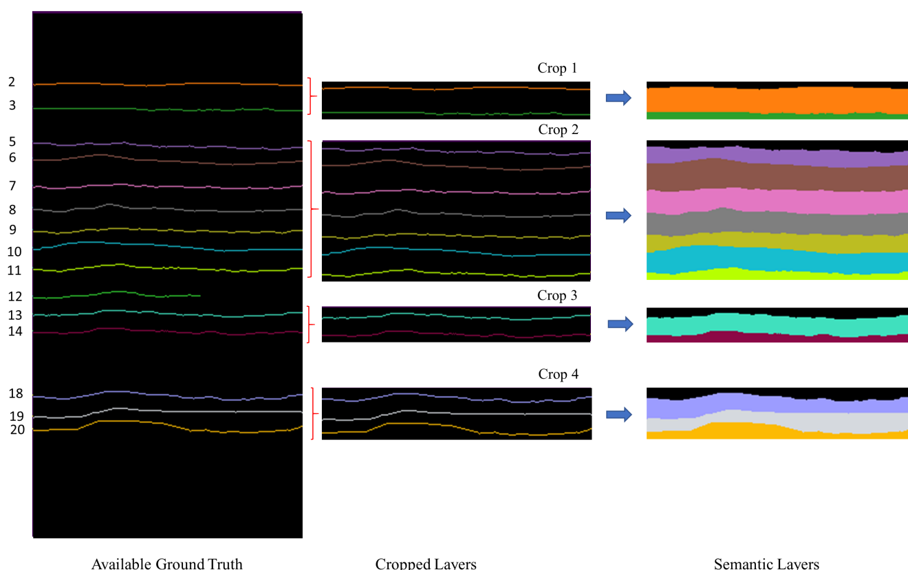
Figure 4. Processing the training labels: We crop out the ‘Available Ground Truth’, into multiple segments, as shown in ‘Cropped Layers’. These cropped portions are then prepared for semantic segmentation, as shown in ‘Semantic Layers’.
