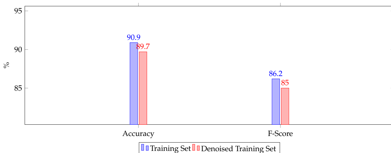
Figure 14. Accuracy and F-1 score obtained over the combined training set and the combined denoised training set.
