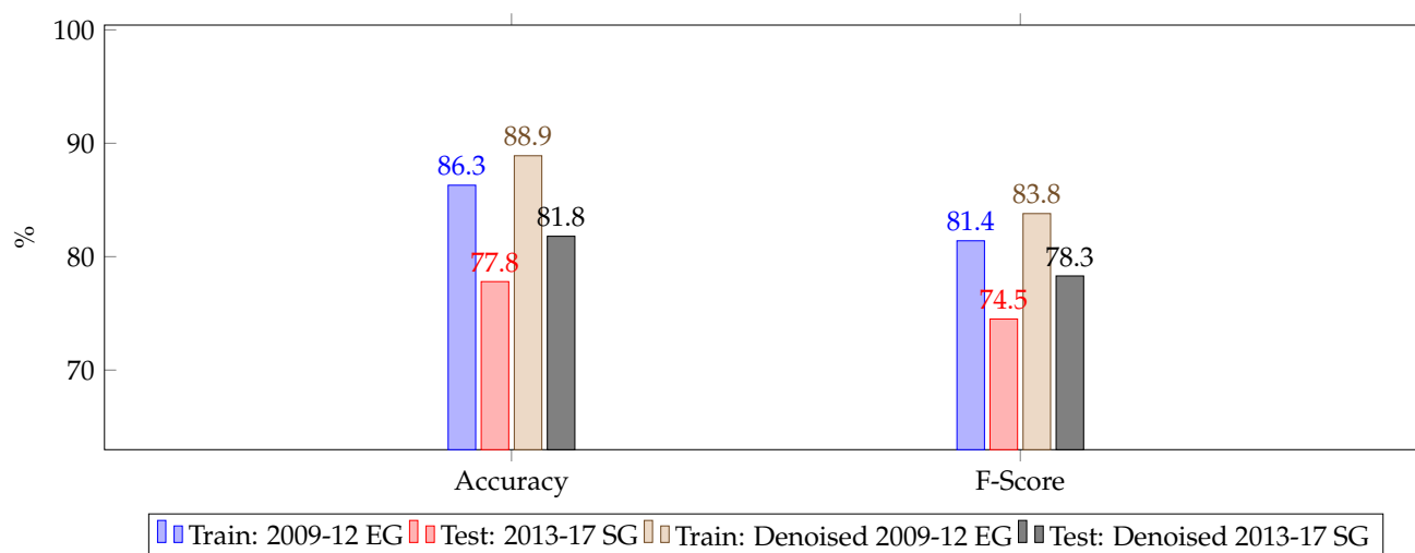
Figure 13. Accuracy and F-score obtained by training on 2009–2012 dataset and testing on 2013–2017 dataset.
