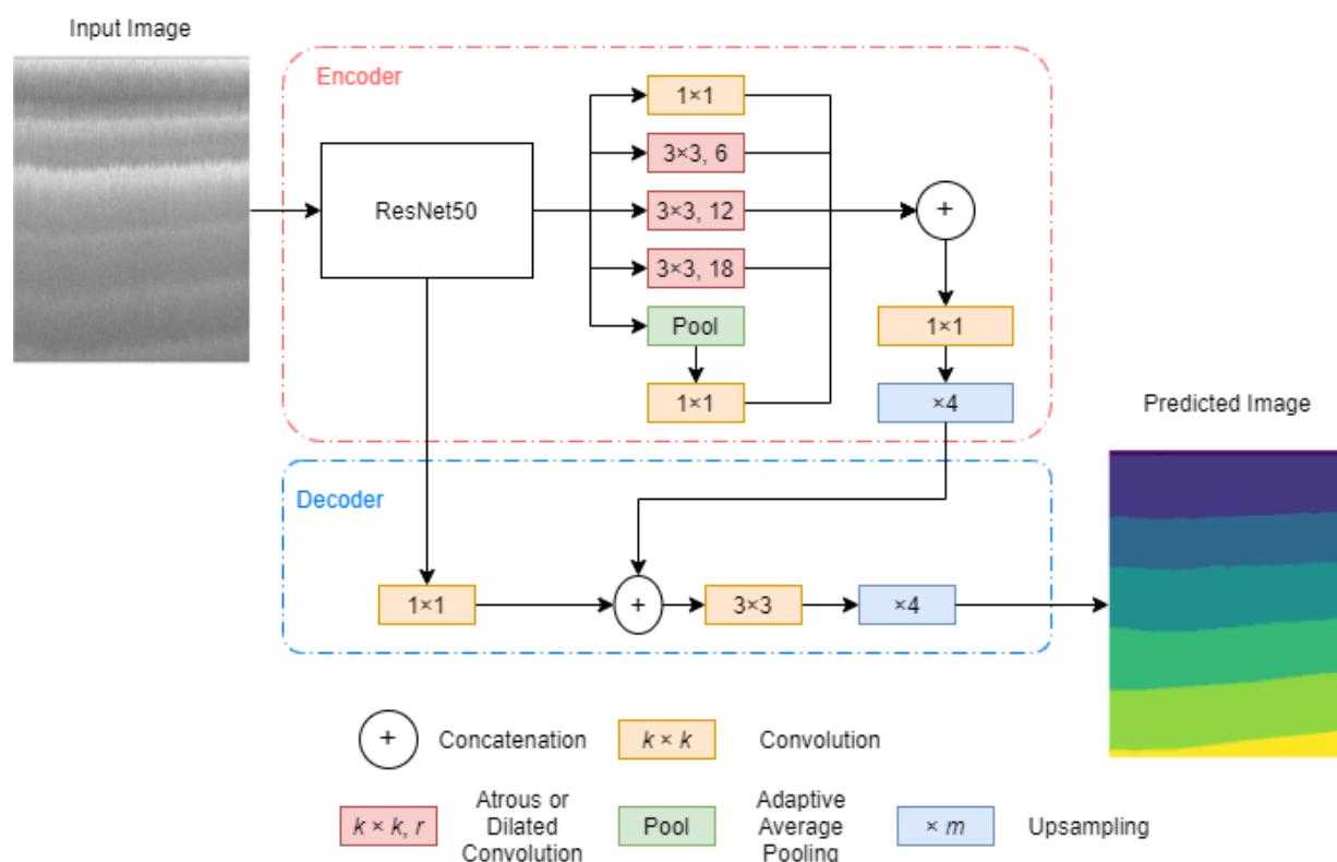
Figure 8. DeepLabv3+ [25] architecture with ResNet50 [31] backbone.
