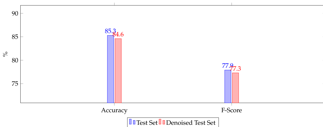
Figure 15. Accuracy and F-1 score obtained over the combined test set and the combined denoised test set.
