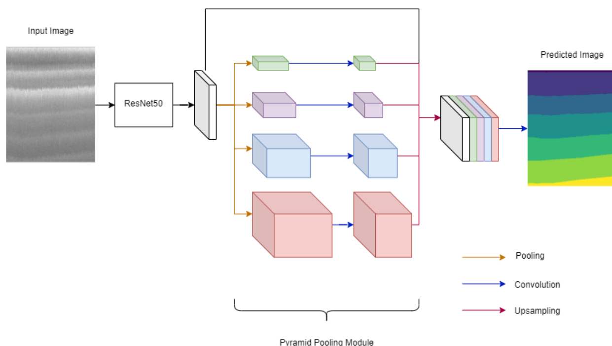
Figure 7. PSPNet [26] architecture.
