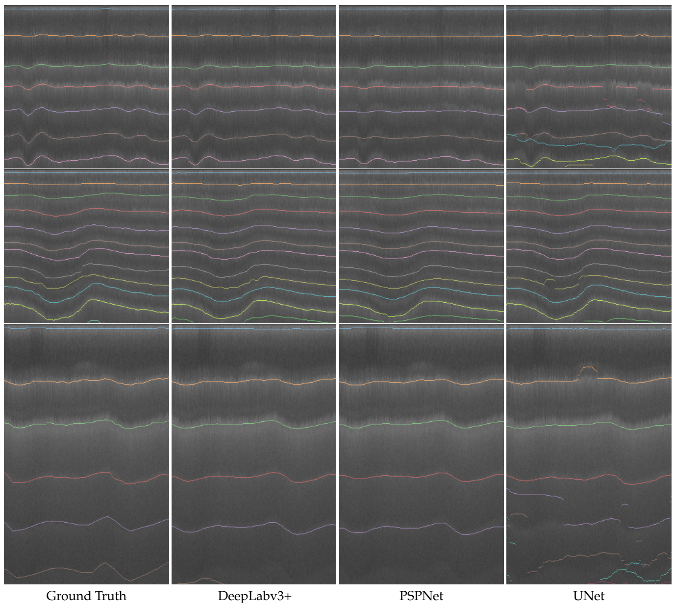
Figure 11. Radar images overlaid with Ground Truth layers ( first column ) and layers predicted from the three FCNs: DeepLabv3+ ( second column ), PSPNet ( third column ), and UNet ( fourth column ). The results shown are from each network's best output in terms of mean IoU (Table 3). More examples are in Figure 12.
