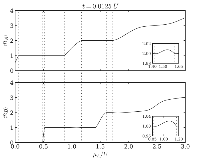
FIG. 4. Densities on two sublattices of the kagome lattice for V = 0.5U and t = 0.0125U [see Fig. 2(b)]. Dotted vertical lines show phase boundaries. Insets show magnified views, with the same axes.
