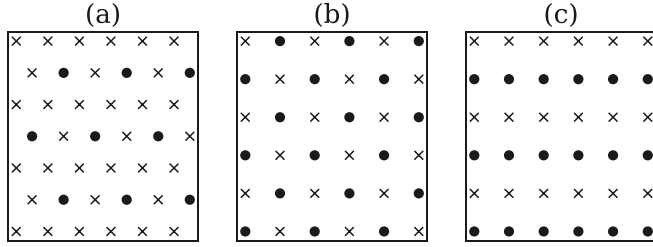
FIG. 1. Example lattices: (a) kagome; (b) checkerboard; (c) stripe. In all cases the local potential is different on the A sublattice, marked by x 's, and the B sublattice, marked by dots.
