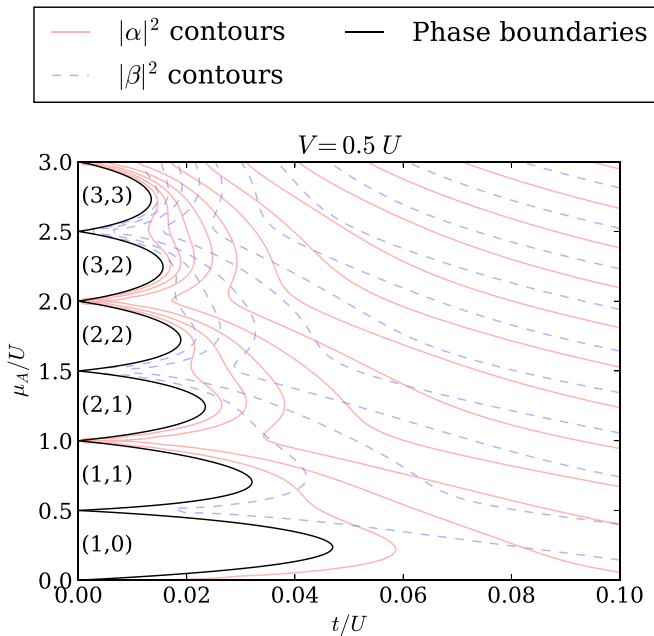
FIG. 3. Phase boundaries for the striped lattice with sublattice bias V = 0.5 . Energies are given in terms of the on-site interaction U . Mott states with n_A and n_B atoms per site on each sublattice are labeled by (n_A, n_B) . Solid (red) curves and dashed (blue) curves denote evenly spaced contours of fixed condensate densities, |\alpha|^2 and |\beta|^2 , with spacing 0.25. In contrast to the kagome lattice, for the striped lattice the lobes are more symmetric.
