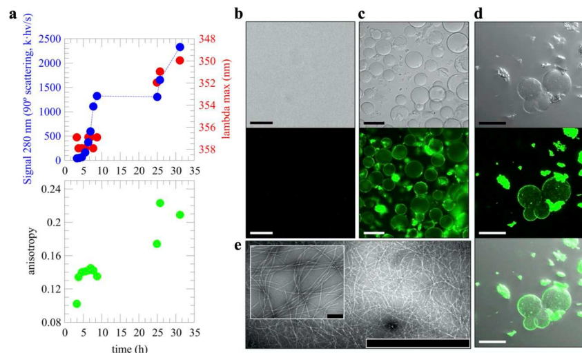
Fig 2. Droplet assembly is coupled to fibril formation. (a) Light scattering following the signal at 280 nm over time (top, blue circles), maximum emission wavelength (top, red circles), and fluorescence anisotropy (bottom, green circles) over time during droplet and fibril formation. (b) The TDP-43's PrLD sample eluted from the column is free of droplets (top). To test for the presence of amyloid fibrils, ThT was added to the sample and visualized by fluorescence microscopy (bottom). The lack of fluorescence indicates that no amyloid fibrils are present at the beginning of the experiments. (c) Aggregated samples (i.e., samples where no signal is detected in LSNMR experiments) present extensive droplet formation, as well as irregularly shaped clumps (top, light transmitted image). Interestingly, both the droplets and the clumps were recognized by ThT (bottom, fluorescent image). These images were collected using fluorescence microscopy on 110 \mu M TDP-43 PrLD. The scale bars in panels a and b are 100 \mu m. (d) Confocal microscopy images of the 55 \mu M aggregated sample (transmitted light, top; fluorescence, middle; overlay, bottom) showing ThT bound to droplets surface as well as to the irregularly shaped clumps, suggesting that the latter are made by amyloid fibrils which are formed and released from the droplet surface. Scale bar is 50 \mu m. (e) TEM micrographs confirmed the presence of amyloid fibrils, in agreement with ThT fluorescence (scale bar: 2 \mu m; at inset image: 200 nm). Numerical data for panel A can be found in S1 Data . PrLD, prion-like domain; TDP-43, Transactive response DNA-binding Protein of 43 kDa; TEM, transmission electron microscopy; ThT, Thioflavin T.
