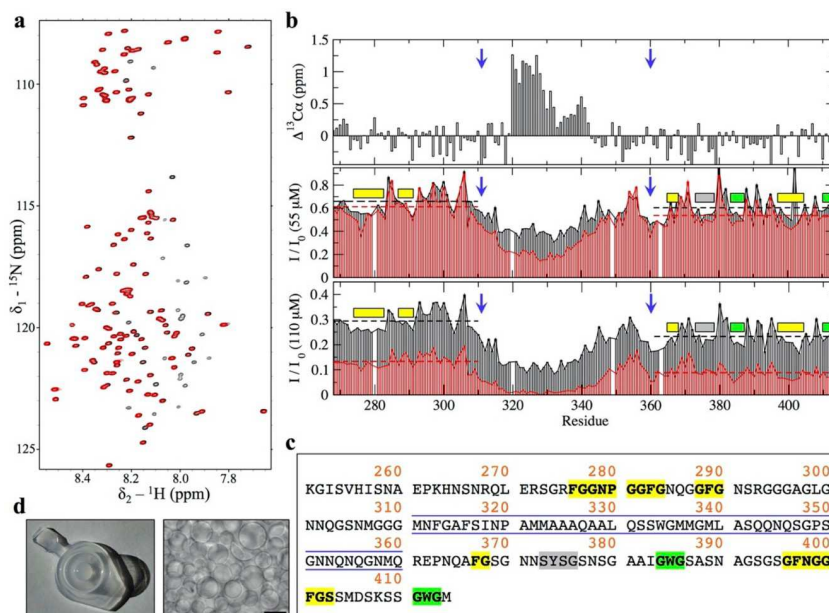
Fig 1. LSNMR characterization of the PrLD of TDP-43's aggregation at low pH. (a) The ^1\text{H} - ^{15}\text{N} HSQC spectra of TDP-43 PrLD at pH 4 and 25^\circ\text{C} (110 \mu\text{M} ), showing a narrow ^1\text{H} amide chemical shift range typical of a disordered region. Black peaks correspond to a spectrum recorded within 1 hour from sample preparation, the time elapsed between column elution and the start of the NMR experiments (see Methods ). The spectrum in red was the last recorded on this sample ( S1 and S2 Tables), where signals corresponding to some but not all residues disappear due to self-association. (b) Signals whose intensity is lost over time correspond to the central region spanning residues 311–360 (delimited by blue arrows), which contain an \alpha -helix as evinced by ^{13}\text{C}_\alpha chemical shifts (top panel). In addition, several short segments within the 2 regions N-terminal and carboxyl terminus to the 311–360 core (i.e., 267–310 and 361–414) also exhibit moderate signal loss, which are consistently observed at 55 \mu\text{M} (middle panel) and at 110 \mu\text{M} (bottom panel). This is illustrated by plotting the intensity values from the first ^1\text{H} - ^{15}\text{N} HSQC ( I_0 , black bars, 1 hour from sample preparation) and those from a ^1\text{H} - ^{15}\text{N} HSQC recorded approximately 20 hours later, plotted as I/I_0 (red bars, I and I_0 correspond to intensity values for the second and first ^1\text{H} - ^{15}\text{N} HSQC, respectively, normalized to the most intense peak). Note that average values for the 2 regions 267–310 and 361–414 N-terminal and carboxyl terminus to the central segment are shown as dashed horizontal lines (black and red colors for the I_0 and I/I_0 data sets, respectively), which highlights that the regions with lower than the average intensities mostly map to segments containing aromatic residues: Phe (yellow boxes), Tyr (gray box), and Trp (green boxes). (c) TDP-43's PrLD sequence illustrating the central region composed of residues 311–360 (blue lines, to match blue arrows in panel b), which was the focus of some earlier studies and contains the helical segment important for assembly, as well as the aromatic residues outside this core (Phe in yellow, Tyr in gray, and Trp in green). (d) At the end of the NMR experiments, the samples were found aggregated (left panel) and displayed extensive droplet formation (right panel, scale bar: 100 \mu\text{m} ). This was imaged on the 110 \mu\text{M} sample. The ^{15}\text{N} - ^1\text{H} HSQC spectra are available from Mendeley Data ( http://dx.doi.org/10.17632/gvy4tc5nky.1 ), and the NMR chemical shifts are deposited in the BMRB under accession code 50154. Numerical data for the 3 plots in panel B can be found in S1 Data . BMRB, Biological Magnetic Resonance Bank; LSNMR, liquid-state NMR; PrLD, prion-like domain; TDP-43, Transactive response DNA-binding Protein of 43 kDa. https://doi.org/10.1371/journal.pbio.3001198.g001
