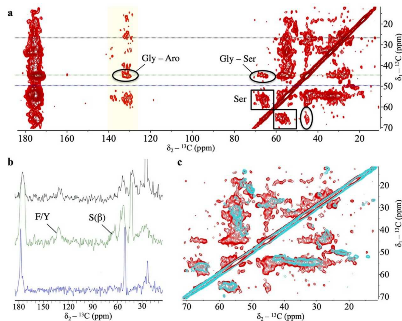
Fig 4. Fibrils from the PrLD of TDP-43 are stabilized by Phe-Gly motifs. (a) Two-dimensional ^{13}\text{C} - ^{13}\text{C} DARR spectrum recorded with a 250 ms mixing time on fibrils formed by the PrLD of TDP-43. This experiment detects residues immobilized within the fibril core. Fibrils are rich in \beta -sheet content, as indicated by the presence of Ser residues showing differences of ^{13}\text{C}\beta - ^{13}\text{C}\alpha > 8 ppm (black boxes). Cross-peaks between Ser and Gly (black ellipses) indicate that Ser-Gly motifs, which are located outside the helical region, are relevant in the fibril form. Signals around 130–140 ppm (yellow shaded region) correspond to aromatic ^{13}\text{C} from Phe/Tyr residues. Considering that there is only 1 Tyr in the PrLD sequence, most cross-peaks arise from Phe ( ^{13}\text{C}\delta/^{13}\text{C}\epsilon )-Gly ( ^{13}\text{C}\alpha ) (black circles). (b) Horizontal slices extracted from the 250 ms DARR shown in a, taken at \delta_1 = 27.03 ppm (in black), which illustrates a crowded region that covers aliphatic, aromatic, and carbonyl peaks; \delta_1 = 45.07 ppm (in green), which is distinctive of Gly ^{13}\text{C}\alpha chemical shift values, illustrating signals contributed by aromatic ^{13}\text{C} nuclei from Phe/Tyr, as well as by ^{13}\text{C}\beta of Ser, as identified by their distinctive chemical shift values. This supports the presence of immobilized Gly, Ser, and Phe residues in the fibril core; and \delta_1 = 49.69 ppm (in blue), which lacks strong resonances thus facilitating an appreciation of the overall signal-to-noise of the SSNMR data. (c) A short mixing time (20 ms) ^{13}\text{C} - ^{13}\text{C} DARR spectrum (in cyan) overlapped onto the 250-ms spectrum from panel a (in red). At this short mixing, only intra-residue contacts are detected, which supports the assignment of sequential contacts that build up at larger mixing times. All these spectra are available from Mendeley Data ( http://dx.doi.org/10.17632/gvy4tc5nky.1 ). DARR, Dipolar Assisted Rotational Resonance; PrLD, prion-like domain; SSNMR, solid-state NMR; TDP-43, Transactive response DNA-binding Protein of 43 kDa.
