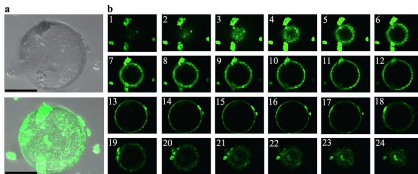
Fig 3. ThT-positive, TDP-43's PrLD fibrils emerge from protein droplets. (a) Visualization of a ThT-stained droplet from the 110 \mu M aggregated sample by confocal microscopy (top: transmitted light image, bottom: overlay with the ThT fluorescent image; scale bar: 50 \mu m). The nonhomogeneous staining suggests that fibril assembly occurs on droplet surface, and not its interior. Scale bar is 50 \mu m. (b) Sections of the droplet evince that the droplet interior is devoid of fibrils, whereas ThT fluorescence maps the droplet surface, at the droplet/solvent interface boundaries, and suggests detachment of fibrils once a certain size is reached. Images 1–24 are selected sections from a collection of 42 slices passing from pole to equator to pole that illustrate the distribution of ThT-positive aggregates across the droplet surface. PrLD, prion-like domain; TDP-43, Transactive response DNA-binding Protein of 43 kDa; ThT, Thioflavin T.
