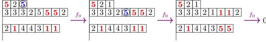
FIGURE 7. The 0-string for a semistandard key tabloid, with 0-paired letters in red and the leftmost unpaired 5 circled.
