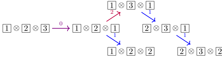
FIGURE 3. The affine Demazure crystal \tilde{\mathcal{B}}_{s_1 s_2 s_0}(1, 1, 1) .
