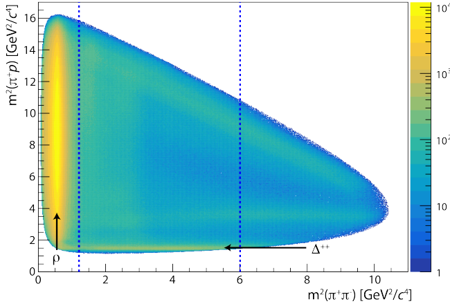
Figure 2. Dalitz plot of products of the reaction \bar{\gamma}p \rightarrow \pi^+\pi^-p . Candidates between dashed lines are selected. Data shown are not efficiency corrected.
