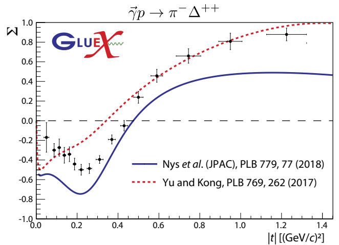
Figure 5. Beam asymmetry \Sigma vs. |t| compared to theoretical predictions. The error bars indicate the statistical and systematic uncertainties combined in quadrature.
