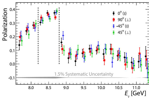
Figure 1. The degree of linear polarization for four different orientations of diamond radiator as a function of beam photon energy, as measured by the TPOL. Events between the dashed lines ( 8.2 \text{ GeV} < E_\gamma < 8.8 \text{ GeV} ) are analyzed. (Data points are slightly offset for clarity.)
