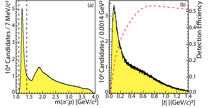
Figure 3. (a) The \pi^+p invariant mass distribution of events satisfying all selection criteria. In addition to the \Delta^{++} , excited states around 1.9 \text{GeV}/c^2 are visible. (b) The distribution of |t| for candidates between the dashed lines in panel (a) and the detection efficiency as a function of |t| . Data plotted are not efficiency corrected.
