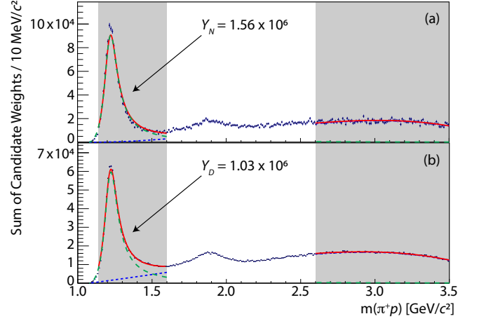
Figure 4. (color online) Fit to (a) numerator N and (b) denominator D defined in Eqs. 5b and 5a, in the extended range 0.4 \text{ (GeV}/c)^2 < |t| < 1.4 \text{ (GeV}/c)^2 . The \Delta^{++} component is shown in green (dashed), polynomial background in blue (dotted), and total fit in red. Data are fit in the shaded regions only, the integral of the green (dashed) curve in the lower shaded region is used to determine the yields Y_N and Y_D .
