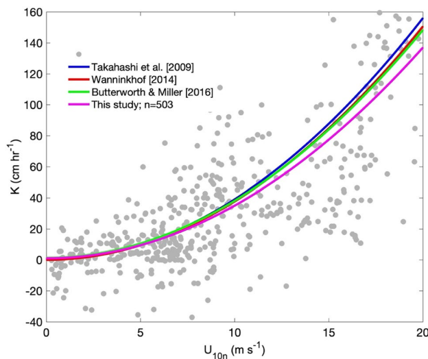
Figure 7. Relationship between the CO 2 transfer velocity coefficient and the neutral wind speed at 10 m calculated from the data collected in this experiment. The quadratic fitted curve K = 0.34 \cdot U_{10n}^2 - 0.32 \cdot U_{10n} + 0.94 with r^2 = 0.75 is represented by the magenta line. The blue, red and green curves represent the CO 2 transfer coefficient obtained in the literature 36,69,70 . MATLAB, Version 9.1.0.441655 (R2016b). https://www.mathworks.com .
