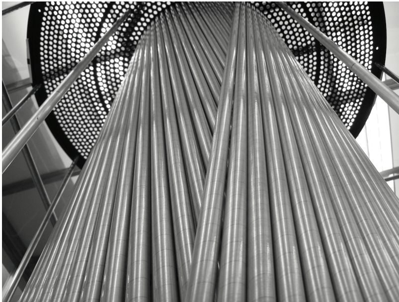
Figure 16: The Central Drift Chamber during construction. A partially completed layer of stereo straw tubes is shown, surrounding a layer of straw tubes at the opposite stereo angle. Part of the carbon fiber endplate, two temporary tension rods and some of the 12 permanent support rods linking the two endplates can also be seen.
