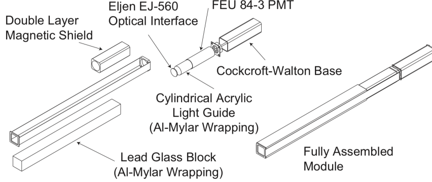
Figure 23: Expanded view of a single FCAL module.
