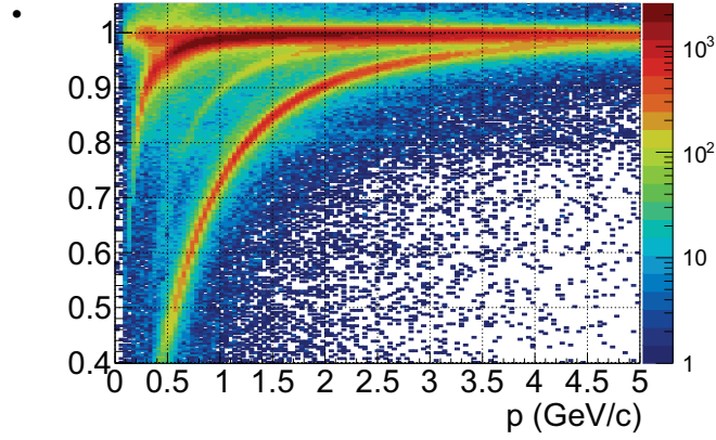
Figure 29: \beta of positive tracks versus track momentum, showing bands for e^+ , \pi^+ , K^+ and p for the TOF detector. The color coding of the third dimension is in logarithmic scale.(Color online)
