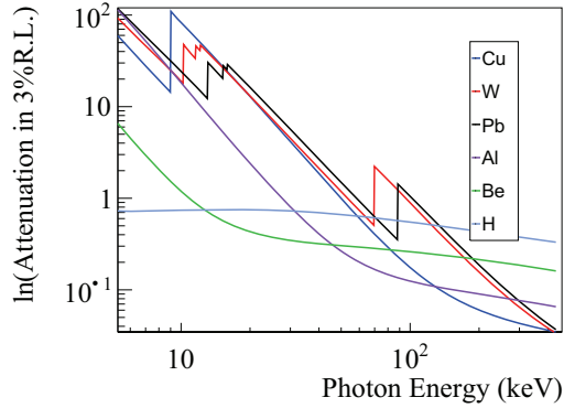
Figure 11: Attenuation of low-energy photons in foils with a thickness of 3% of a radiation length for different materials as a function of photon energy. The W foil was selected to reduce the random background hits in the detector drift chambers. The attenuation coefficients are taken from Ref. [20].
