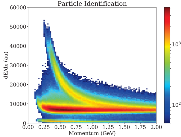
Figure 28: dE/dx vs. p for the Start Counter. The curved band corresponds to protons while the horizontal band corresponds to electrons, pions, and kaons. Pion/proton separation is achievable for tracks with p < 0.9 GeV/ c .
