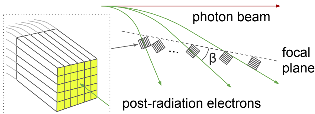
Figure 9: Conceptual overview of the tagger microscope design, showing the fiber bundles and light guides (left), and the orientation of these bundles aligned with the incoming electron beam direction in the tagger focal plane (right). The variation of the crossing angle \beta is exaggerated for the sake of illustration.
