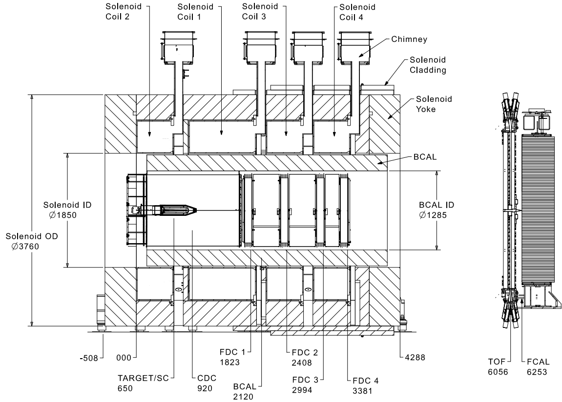
Figure 3: GlueX spectrometer layout. Dimensions are given in mm. The numbers show the Z-coordinates of the detectors' centers, or of the front face of the FCAL modules. Glossary: SC - Start Counter (Section 8.1), CDC - Central Drift Chamber (Section 5.1), FDC - Forward Drift Chamber (Section 5.2), BCAL - Barrel Calorimeter (Section 7.1), TOF - Time-of-Flight hodoscope (Section 8.2), FCAL - Forward Calorimeter (Section 7.2).
