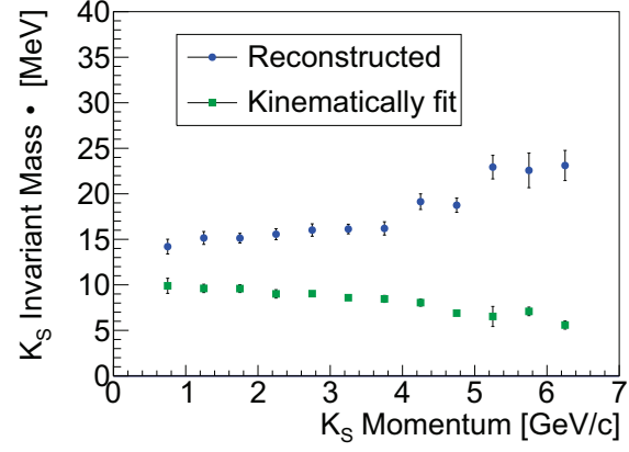
Figure 49: K_S \rightarrow \pi^+\pi^- invariant mass resolution for the events shown in Fig.48, as a function of K_S momentum, both before and after a kinetic fit, which constrains energy and momentum conservation. (Color online)
