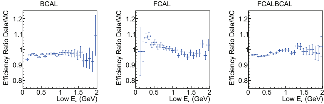
Figure 44: Ratios of relative photon reconstruction efficiency between data and simulation determined from \pi^0 \rightarrow \gamma\gamma decays in \gamma p \rightarrow \pi^+\pi^-\pi^0 p events. The efficiency ratios are shown for the cases where (left) both photons were measured in the BCAL, (middle) both photons were measured in the FCAL, and (right) one photon was measured in the BCAL and the other in the FCAL.
