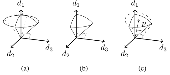
Figure 2: Illustrations of the gradient pruning method by directional-preferences. (a) The cone \mathcal{F}(d_1, \gamma) is the possible gradient directions. (b) The quarter cone is the possible gradient directions after the queries. (c) The dashed cone \mathcal{F}(p, \gamma') overapproximates possible gradient directions.
