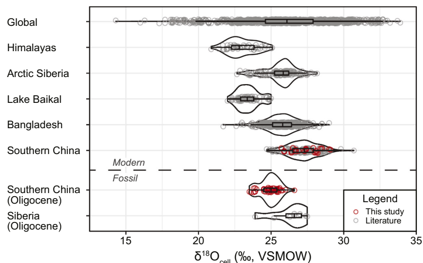
Fig. 3. Violin plots with \delta^{18}\text{O}_{\text{cell}} data points, box plots, and kernel densities for modern and fossil samples. Late Oligocene values for Siberia and southern China have both been corrected by +2.5\% to account for changes in seawater composition. Global data include compilations by Sternberg et al. (2007) and Richter et al. (2008b), with updated sites including a high elevation site in the Himalayas (Xu et al., 2018), high latitude site in arctic Siberia (Holzkämper et al., 2008), inland/high latitude site in Lake Baikal (central Russia; Tartakovsky et al., 2012), and Bangladesh (Islam et al., 2021). Fossil data from Siberia are from Richter et al. (2008a). Box plots show the first through third quartiles with whiskers extending a distance of the interquartile range on either side of the box. All new modern data sets were trimmed to the most recent 50 years for each \delta^{18}\text{O}_{\text{cell}} series to prevent overweighting individual sites. Data were available as supplementary materials from the primary publications. Data used in this figure are available in the supplementary materials (Table S1).
