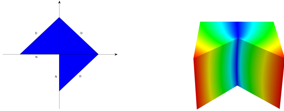
Figure 4: Example 8.1 (two Neumann faces): the top view of \Omega_p , top Dirichlet face marked in blue (left); the absolute value of the numerical solution (right).
