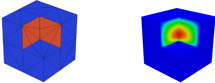
Figure 7: Example 8.4 (three singular edges in a Fichera domain): Neumann faces marked in red and Dirichlet faces in blue (left); the numerical solution (right).
