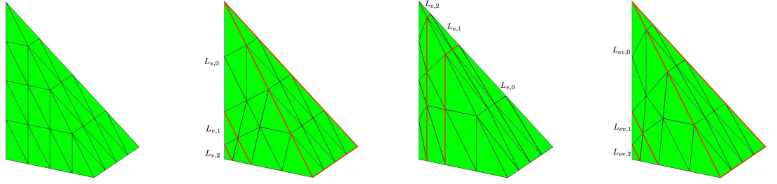
Figure 2: Anisotropic triangulations after two consecutive refinements and mesh layers on an initial tetrahedron (left – right): o -tetrahedron, v - or v_e -tetrahedron ( \kappa = 0.3 ), e -tetrahedron ( \kappa_e = 0.3 ); ev -tetrahedron ( \kappa_{ec} = \kappa_c = 0.3, \kappa_e = 0.4 ).
