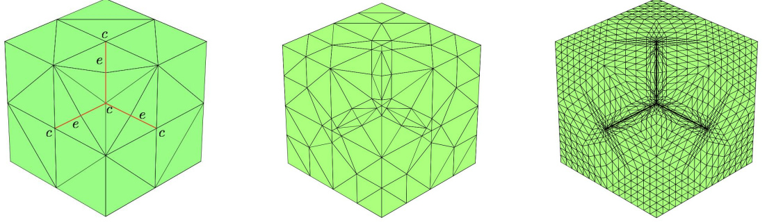
Figure 8: Graded meshes on the Fichera domain (left-right): the initial mesh, mesh after one refinement, mesh after three refinements ( \kappa_e = \kappa_c = 0.2 ).
