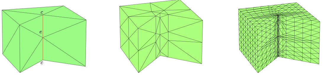
Figure 3: Graded meshes on the prism domain (left – right): the initial mesh, mesh after one refinement, mesh after three refinements ( \kappa_e = \kappa_c = 0.2 ).
