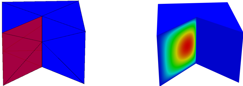
Figure 6: Example 8.3 (a DN singular edge): Neumann face marked in red and Dirichlet face in blue (left); the numerical solution (right).
