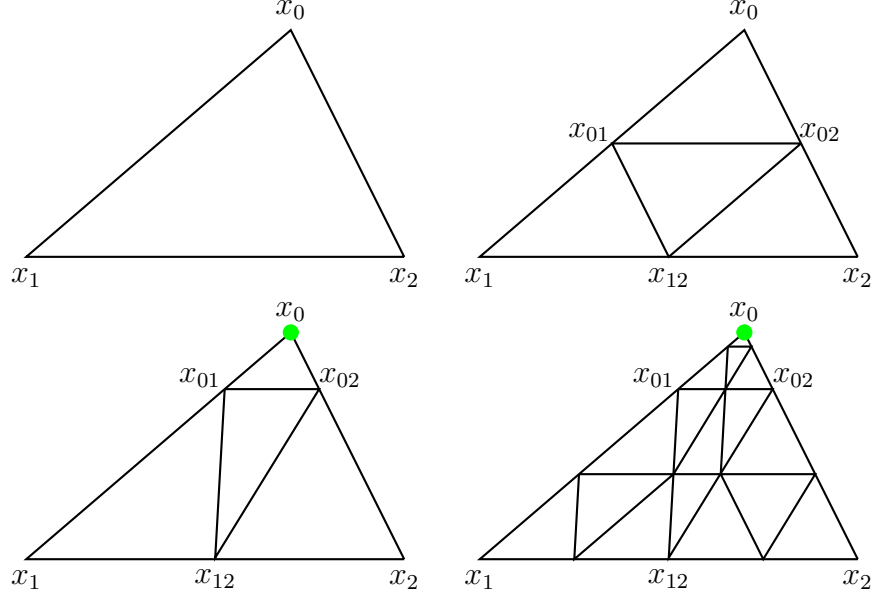
FIGURE 5. Refinement of a triangle \triangle x_0x_1x_2 . First row: (left – right): the initial triangle and the midpoint refinement; second row: two consecutive graded refinements toward x_0 = Q , ( \kappa < 0.5 ).
