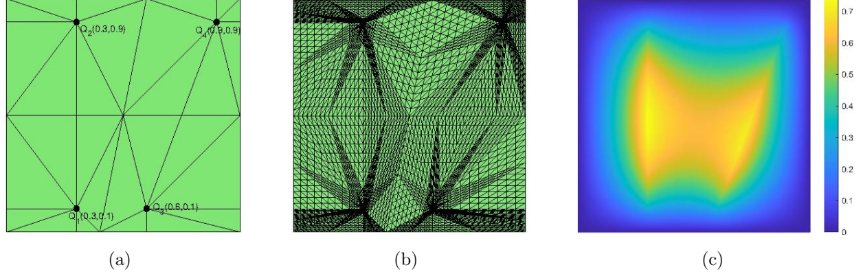
FIGURE 10. Graded meshes with two line fractures \gamma_1 = Q_1Q_2 and \gamma_2 = Q_3Q_4 . (a) the initial mesh; (b) the mesh after four refinements, \kappa = \kappa_{Q_1} = \kappa_{Q_2} = \kappa_{Q_3} = \kappa_{Q_4} = 0.2 ; (c) the numerical solution.
