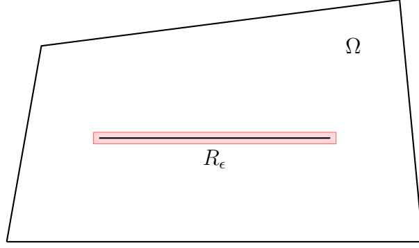
FIGURE 3. A small neighborhood R_\epsilon of the line fracture \gamma .
