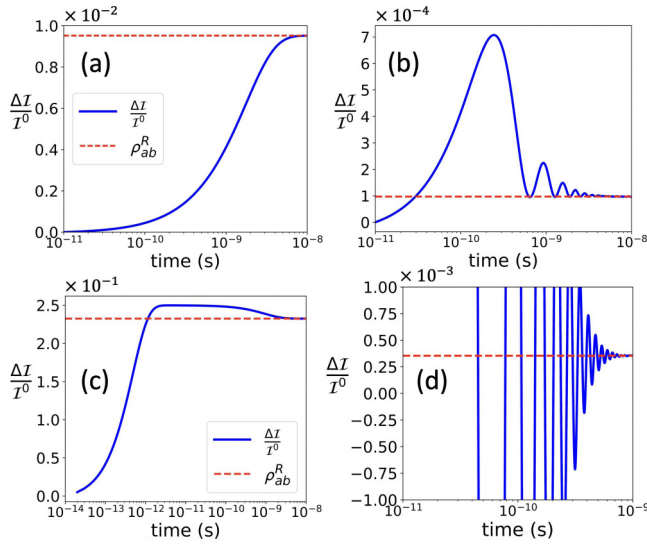
FIG. 7. (a) The ratio of fluorescence intensities calculated for Ca atoms driven by x -polarized vs isotropic incoherent light in different regimes: (a) \bar{n} = 10^{-2} and \Delta/\gamma = 10^{-1} ; (b) \bar{n} = 10^{-2} and \Delta/\gamma = 10 ; (c) \bar{n} = 10^3 and \Delta/\gamma = 10 ; (d) \bar{n} = 10 and \Delta/\gamma = 10^2 . The spontaneous decay lifetime used in the calculations is \tau_s = 1/\gamma = 10^{-9} s.
