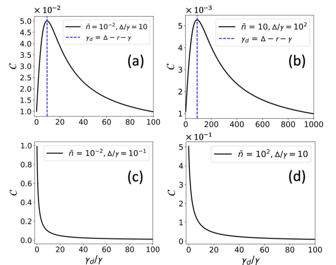
FIG. 6. Steady-state coherence-to-population ratio \mathcal{C} plotted as a function of dimensionless decoherence rate \gamma_d/\gamma in the weak-pumping limit [(a) and (c)] and in the strong-pumping limit [(b) and (d)]. The values of the \Delta/\gamma are indicated in each panel.
