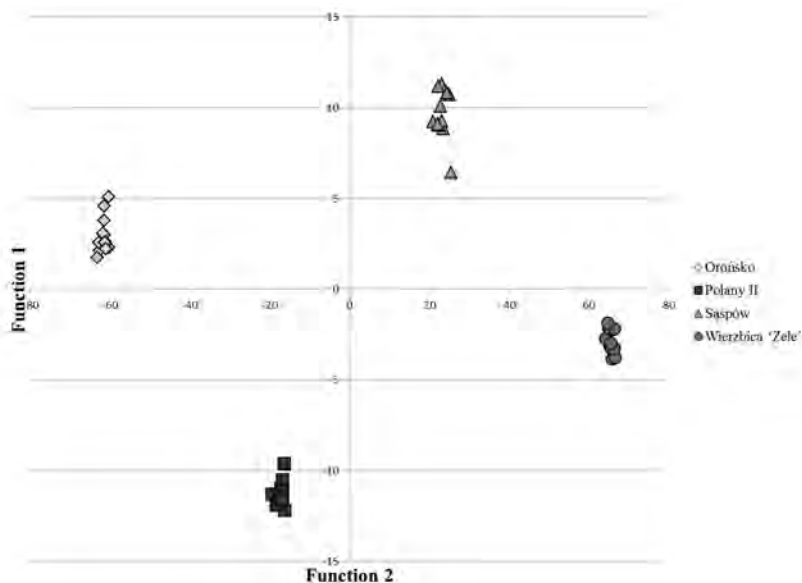
Fig. 3. Discriminant function scatter plot depicting clear separation between all three deposits of 'chocolate' flint (Orońsko, Szydłowiec distr., Wierzbica 'Zeł' and Polany II, Radom distr.) and Jurassic-Cracow (Sąspów, Cracow distr.) flint. Computer graphics: R.M. Parish.
