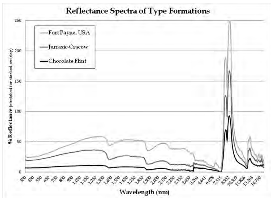
Fig. 1. Overlaid spectra in the visible, near, and middle-infrared of the three material types analysed in the study. Note the similarity of the spectral features. Spectra stacked for visibility.
