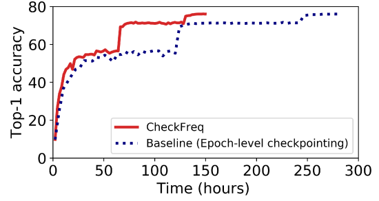
Figure 8: End-to-end training. We train Resnet50 using a Conf-Pascal GPU with interruptions every 5 hours. CheckFreq trains to state-of-the-art accuracy (76.1%) 2\times faster than epoch-based checkpointing by reducing recovery time.
