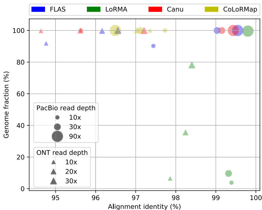
Fig. 1 Correction performance with respect to different long read sequencing depths The alignment identity and genome fraction of yeast PacBio and ONT corrected subsamples generated by CoLoRMap, FLAS, LoRMA and Canu are shown in the figure
