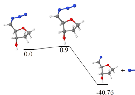
Figure 8. Dissociation of (S'-CH • )-N 3 to S'-CH=N • and N 2 in the gas phase with a small activation barrier of only 0.9 kcal/mol. The geometries of these radicals were optimized, and relative energies (kcal/mol) were calculated by the B3LYP/6-31G** method.
