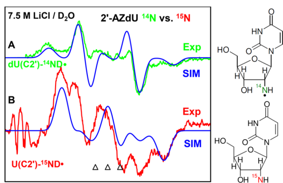
Figure 1. 77 K EPR spectrum of RNH· (U(C2')- 14 ND·) formed via electron-induced attachment in an aqueous glassy (7.5 M LiCl/D 2 O) sample of (A) unlabeled 2 , green color, and (B) 15 N labeled 2 , red color, after visible illumination of each sample by using a photoflood lamp at 77 K for 15 min to remove the uracil anion radical by photoejection of the excess electron. The simulated spectra (blue) (for simulation parameters, see text) are superimposed on the top of the each experimentally recorded spectrum. The three reference markers (open triangles) in this figure and in other figures show the position of Fremy's salt resonance with the central marker at g = 2.0056 . Each of these markers is separated from each other by 13.09 G.
