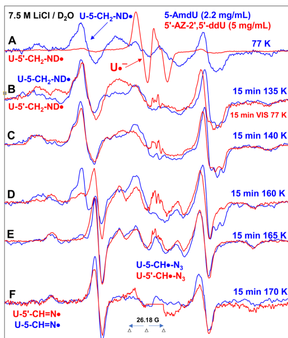
Figure 4. Spectra (A–D) in red were obtained from samples of S' -AZ-2', S' -ddU ( 5 ) ( [S] = 5 mg/mL) after subtraction of the \text{Cl}_2\cdot^- spectrum 7–9,49 from the individual experimentally recorded spectrum. (A) EPR spectrum (red) after radiation-produced prehydrated one-electron addition to the same sample of 5 at 77 K in 7.5 M LiCl/D 2 O. Spectrum (B, red) was obtained after 15 min photoexcitation by a photoflood lamp at 77 K. Spectra (C, red) to (F, red) were obtained via stepwise annealing of the sample for 15 min at 140, 160, 165, and 170 K. All spectra were recorded at 77 K. Sum of two isotropic \beta -proton couplings is assigned to the central doublet (ca. 90.5 G) found in red spectra (A) to (D); the large central doublet (ca. 82 G) in spectra (D–F, red) is due to one isotropic \beta -proton coupling. Meanwhile, the wings in spectra (A)–(F) show the A_{zz} components of the anisotropic nitrogen hyperfine coupling. All spectra were recorded at 77 K. The experimental spectra from AmdU from ref 7 (2.2 mg/mL, blue) are superimposed in (A)–(F) for comparison.
