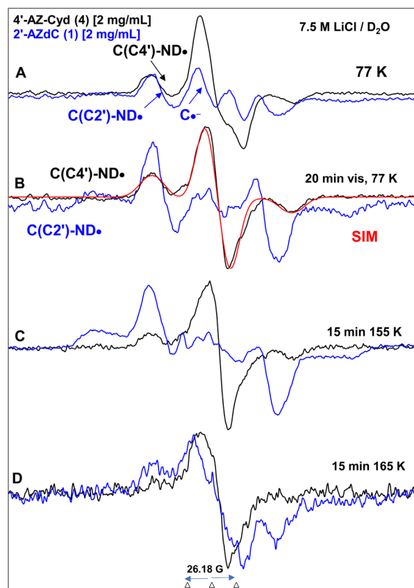
Figure 7. EPR spectra of matched samples of 4'-AZ-C (4, black) and 2'-AZdC (1, blue, 1 also shown in Figure 5) at the native pD (ca. 5) of the homogeneous glassy solution of 7.5 M LiCl in D 2 O after subtraction of the Cl 2 •− spectrum 7–9,49 from the individual experimentally recorded spectrum. (A) After \gamma -irradiation (absorbed dose = 500 Gy) produced one-electron addition at 77 K. (B) After visible illumination of samples employing a photoflood lamp at 77 K for 20 min. The central doublet in both spectra due to the cytosine anion radical (C •− ) is removed by photoejection of the excess electron. The simulated spectrum of C(C4')-ND • is also shown (for simulation parameters, see text). Spectra (C) and (D) are obtained after subsequent annealing for 15 min in the dark at ca. 155 K and at ca. 165 K. All EPR spectra shown in (A)–(D) were recorded at 77 K.
