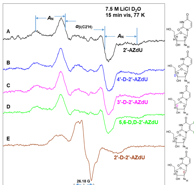
Figure 2. EPR spectra of the aminyl radicals (dU(C2')-ND·) found in matched samples (1 mg/mL of each compound) via radiation-produced (absorbed dose = 500 Gy at 77 K) one-electron addition at 77 K of the homogeneous glassy solution of 7.5 M LiCl in D 2 O after visible illumination of each sample by using a photoflood lamp at 77 K for 15 min to remove the uracil anion radical by photoejection of the excess electron of (A) 2'-AZdU ( 2 ), (B) 4'-D-2'-AZdU ([4'-D]- 2 ), (C) 3'-D-2'-AZdU ([3'-D]- 2 ), (D) 5,6-D, D-2'-AZdU ([5,6-D,D]- 2 ), and (E) 2'-D-2'-AZdU ([2'-D]- 2 ). The extent of \beta -hyperfine coupling by H2' atom and the anisotropic nitrogen hyperfine coupling A_{||} in U(C2')-ND· of 2'-AZdU are represented by stick diagrams.
