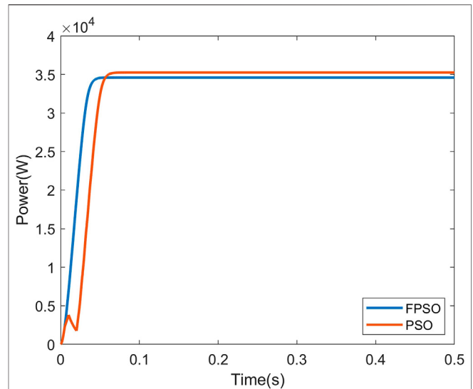
FIGURE 11 | Startup response of the fuzzy adaptive PSO and the conventional PSO MPPT for irradiation 4.
