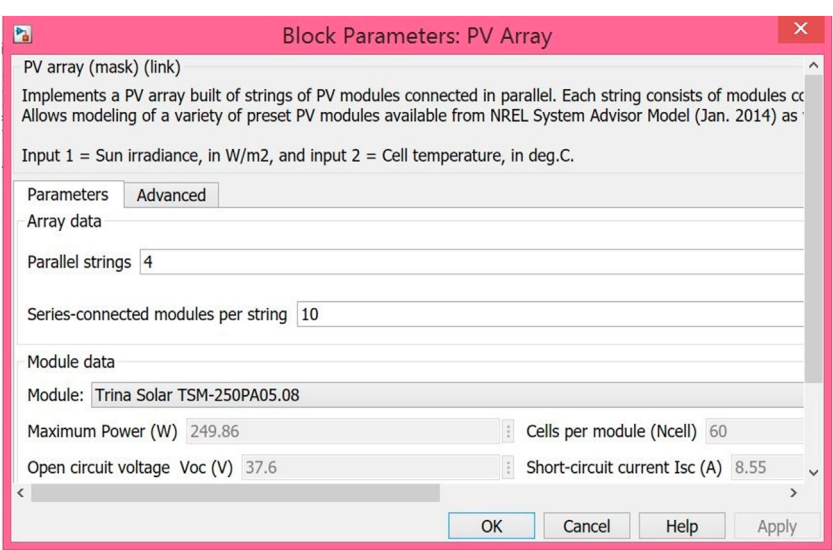
FIGURE 6 | Parameter Configuration of PV arrays.
