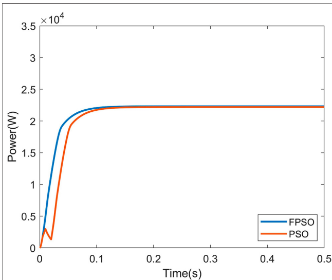
FIGURE 9 | Startup response of the fuzzy adaptive PSO and the conventional PSO MPPT for irradiation 2.
