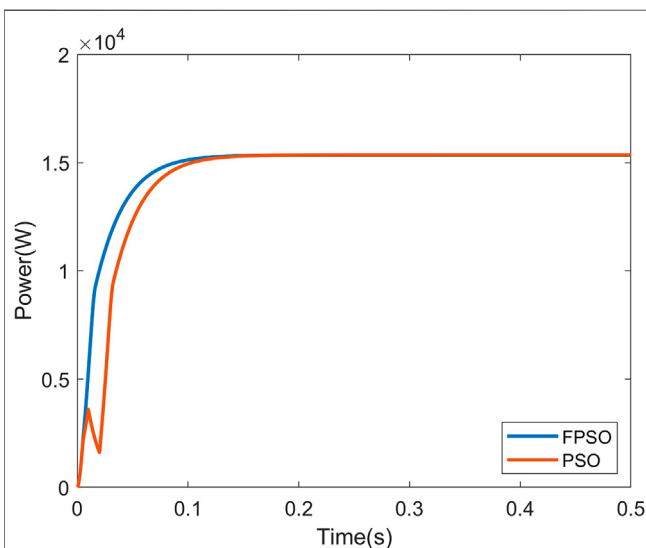
FIGURE 10 | Startup response of the fuzzy adaptive PSO and the conventional PSO MPPT for irradiation 3.
