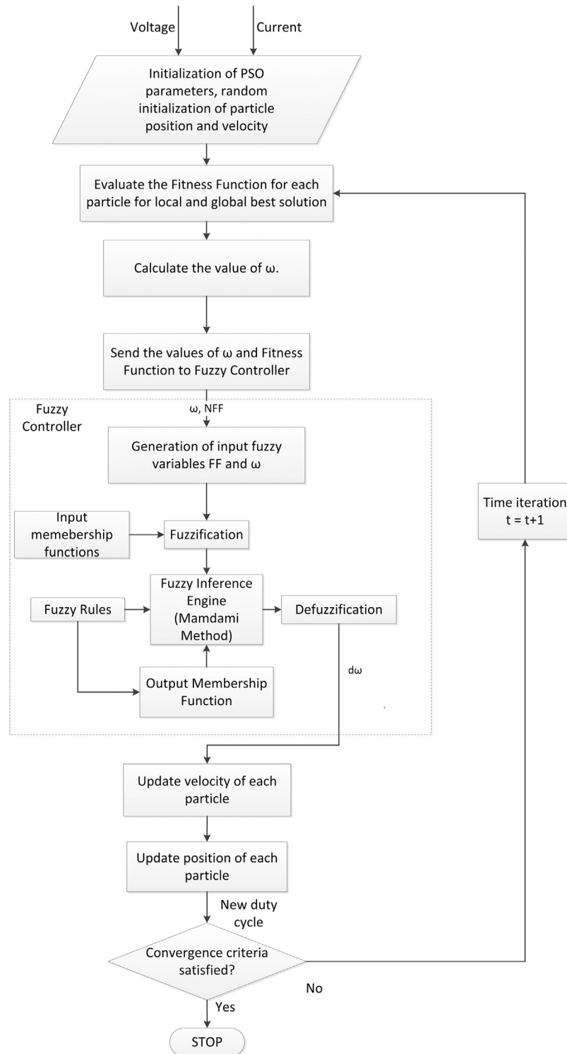
FIGURE 2 | Flowchart of the proposed fuzzy adaptive PSO controller.
