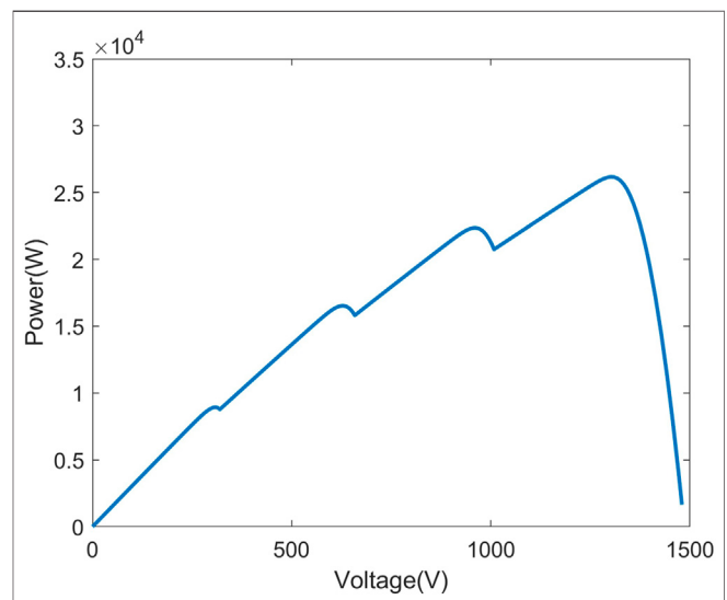
FIGURE 12 | PV curve for irradiation 2.
