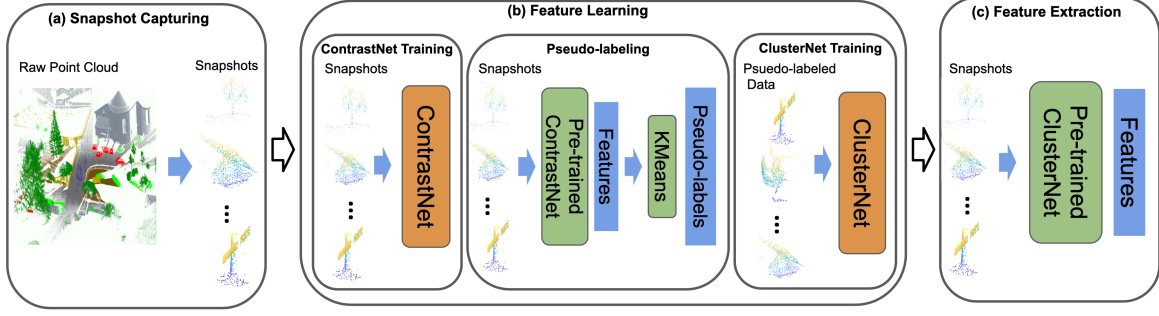
Figure 2: The Snapshot-based self-supervised feature learning pipeline: (a) Snapshot sampling from raw point cloud; (b) Feature learning by part contrasting, snapshot clustering and cluster classification; (c) Snapshot feature extraction by the previously trained ClusterNet.
