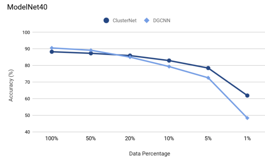
Figure 3: Comparison of the classification accuracies between the ClusterNet and DGCNN on decreasing numbers of labeled data from the ModelNet40
