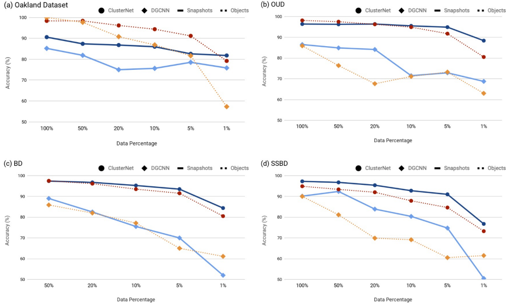
Figure 4: Comparison of the snapshots and objects classification accuracies between the ClusterNet and DGCNN on decreasing numbers of labeled data on complex scene point cloud datasets. The OUD, BD, and SSBD are three sampling configurations derived from the Semantic3D benchmark. Solid lines are results on the snapshots and dotted lines represent the objects.
