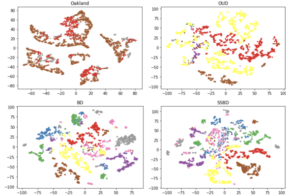
Figure 5: Visualization of the feature embedding of the snapshots from the Oakland dataset and the three Semantic3D configurations. The clusters are colored on the labels for visualization.
