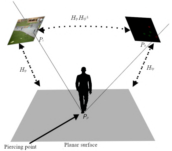
Figure 7: The homography between two images induced by a world plane (the concatenation of two homography matrices).
