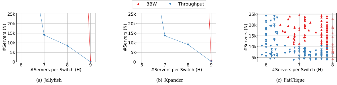
FIGURE 8: Full-throughput Frontier Curve. Uni-regular topologies with H=8 and H=7 can not scale well while preserving full throughput even though they maintain full BBW up to a very large size.
