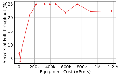
FIGURE A.2: Topology Cost (Jellyfish vs Fat-tree). The relative difference of the maximum servers supported at full throughput (per TUB) between Jellyfish and Fat-tree built with the same equipment using {14, 24, 32, 48, 56, 64, 68, 72, 78, 84, 90, 98}-port switches averaged over 5 runs.
