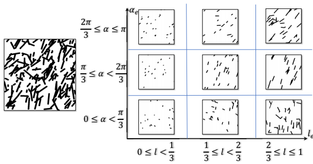
Fig. 4 The extracted edges (left) are divided into 3 \times 3 bins that quantize them according to their length and angle
