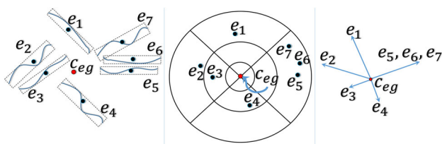
Fig. 5 Edge group representation. Each edge group has its center c_{eg} and a set of edges ( e_1, e_2, \dots, e_7 ) (left). The edge centers are discretized into a grid in polar coordinates centered around c_{eg} (middle). The edge group is represented by the non-empty cells (right), and each cell stores its distance from c_{eg} , the angle, and the list of corresponding edges
