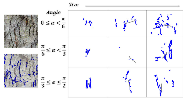
Fig. 6 From the input (left top), we extract edges and group them (left bottom). Then, all edge groups are encoded based on their angles and sizes. The user can control the number of bins
