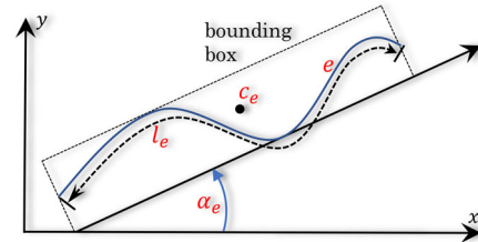
Fig. 3 Detected edge and the features used for further classification: angle \alpha , length l , and center of its bounding box c . We also store the average edge width w
