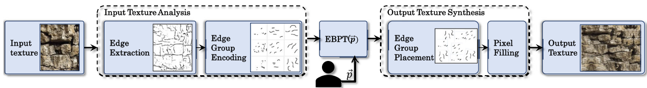
Fig. 2 System overview. The input texture analysis results in the edge-based procedural model for the give input texture image. The input texture is analyzed by extracting and organizing edges into edge groups. Edge groups form the EBPT and are basic building blocks that can be
