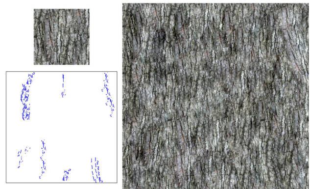
Fig. 11 A small input texture of bark (left up) was used to generate larger texture (right) by placing and randomizing edge groups (left bottom)
