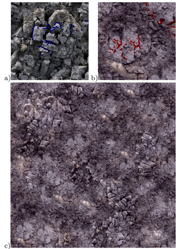
Fig. 14 Combining two EBPTs allows generation of textures from different input. Here, the edge groups from two textures were combined into a new image. Our interactive method grants users direct controls on features of interest. The result (c) consists of background (b) and user-placed features (a)
