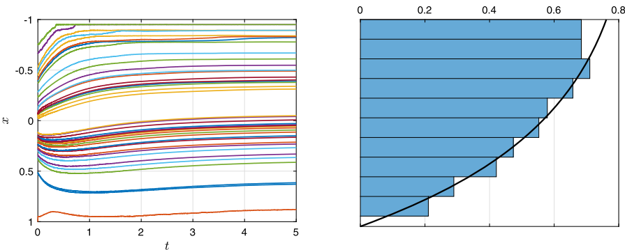
FIG. 3. Evolution of the value of 40 weights chosen at random and histogram of their empirical distribution at time t = 5 .
