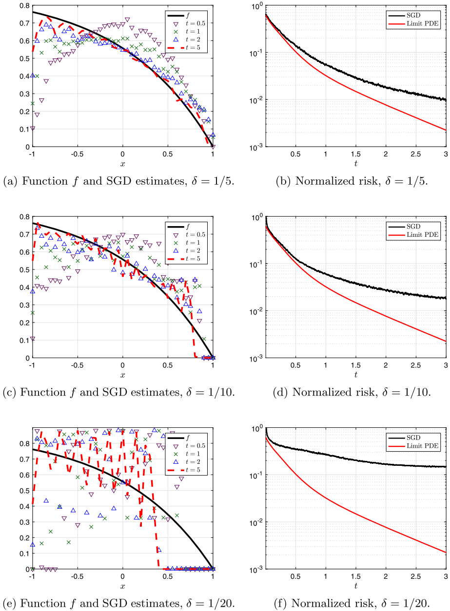
FIG. 8. Dynamics of SGD update (3.5) at different times t and for different values of \delta when the number of neurons is too small ( N = 20 ).
