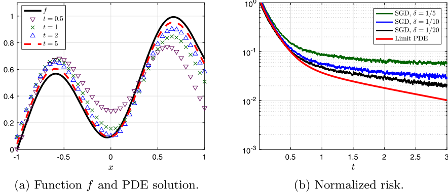
FIG. 7. Dynamics of limit PDE (3.12) at different times t for a nonconcave target function f .
