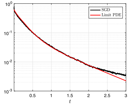
(f) Normalized risk, \delta = 1/20 .
