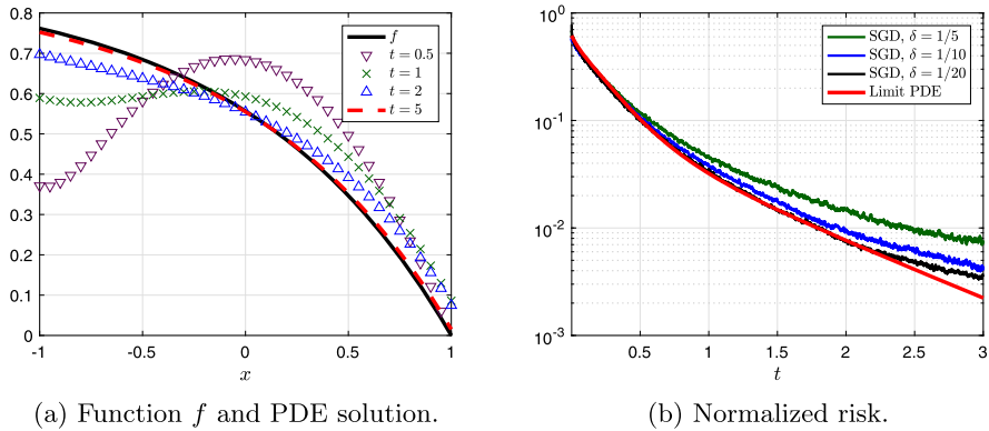
FIG. 2. Dynamics of limit PDE (3.12) at different times t .
