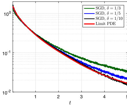
FIG. 4. Normalized risk of SGD for different values of \delta compared with that of the limit PDE for a two-dimensional example.
