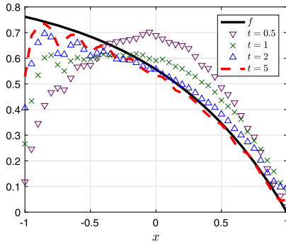
(a) Function f and SGD estimates, \delta = 1/5 .
