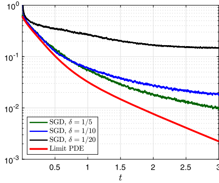
FIG. 9. Normalized risk of the limit PDE (3.12) and of the SGD update (3.5) when the number of neurons is too small ( N = 20 ).
