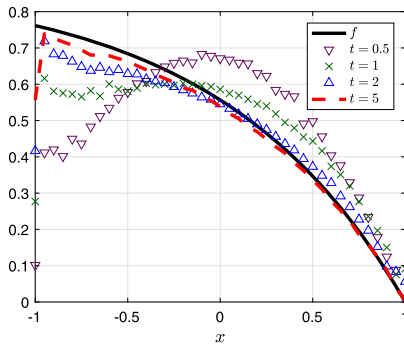
(e) Function f and SGD estimates, \delta = 1/20 .
