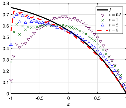
(c) Function f and SGD estimates, \delta = 1/10 .
