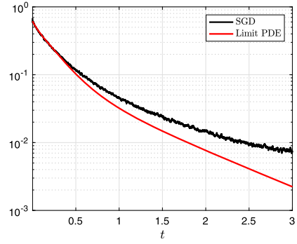
(b) Normalized risk, \delta = 1/5 .
