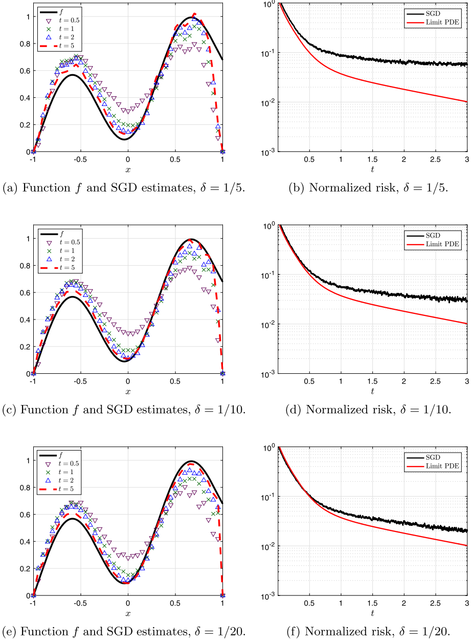
FIG. 6. Dynamics of SGD update (3.5) at different times t and for different values of \delta for a nonconcave target function f .
