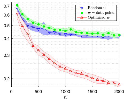
(a) N = 200 , n varies on the x -axis.
