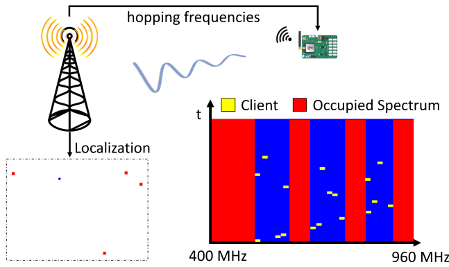
Figure 1: OwLL enables accurate outdoor LoRa localization using TV whitespace bands. We use a TDOA based approach where a LoRa client hops multiple frequencies spanning a wide bandwidth at TV whitespaces and ISM bands
