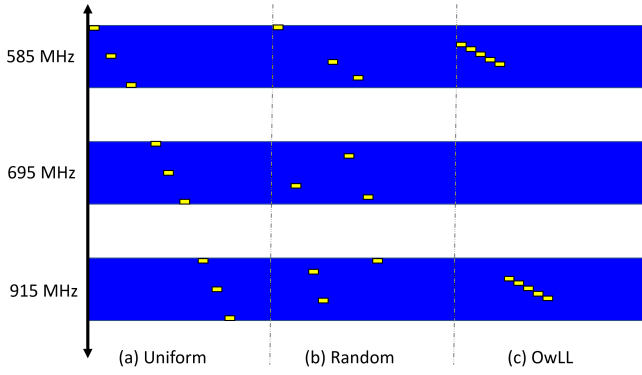
Figure 4: OwLL's approach to select initial frequencies.
