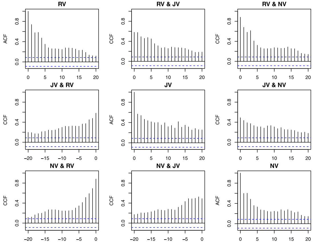
Fig. 2. Auto-correlation function (ACF) and cross-correlation function (CCF) plots (Brockwell and Davis, 2016) for the time series of the daily jump-adjusted MSRV (RV) estimators, the daily jump variation (JV) estimators and the daily nonparametric volatility (NV) estimators with option data.
