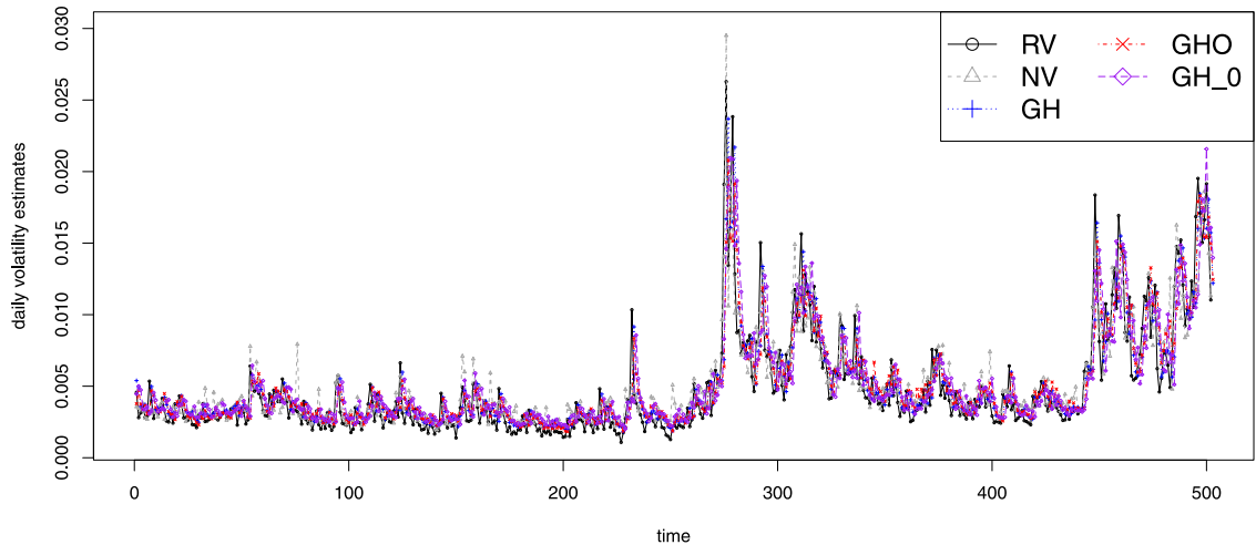
Fig. 3. Daily volatility estimates with (1) RV: jump-adjusted MSRV estimates \sqrt{RV_i} ; (2) NV: option-based nonparametric volatility estimates: \sqrt{NV_i} ; (3) GH: realized GARCH volatility estimates \sqrt{h_i(\hat{\theta}^{GH})} with the QMLE-HL; (4) GHO: realized GARCH volatility estimates \sqrt{h_i(\hat{\theta}^{GHO})} with the QMLE-HLO; (5) GH_0: GARCH volatility estimates \sqrt{h_{i0}(\hat{\theta}_0^{GH})} given the unified GARCH-Itô model..
