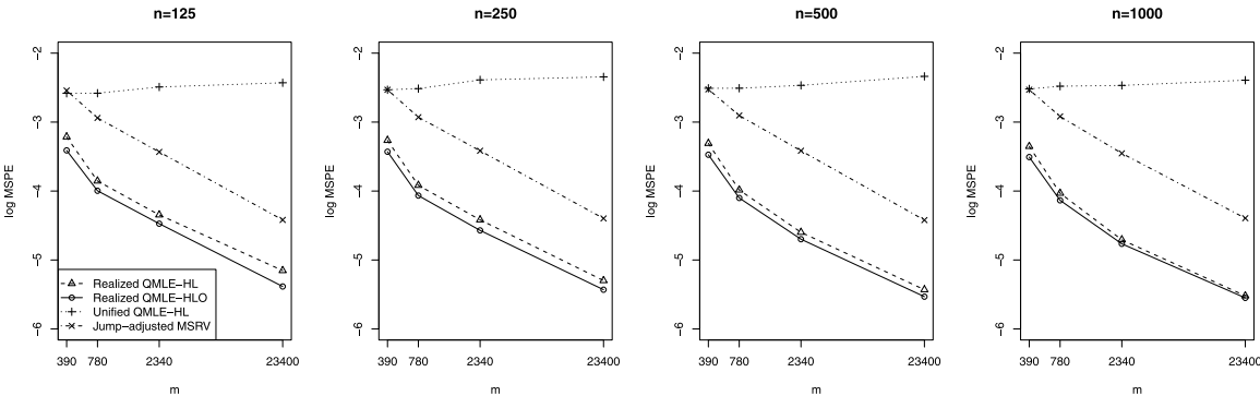
Fig. 1. The log mean squared prediction errors (MSPEs) of the realized GARCH volatility predictors h_i(\theta) , the GARCH volatility predictors h_{i0}(\theta_0) and the benchmark jump-adjusted MSRV predictors RV_{i-1} against m for the different n choices.
