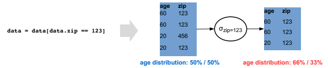
Figure 1: Example: mlinspect identifies relational and ML preprocessing operations in Python code, and instruments them with inspections that check for data distribution bugs.
