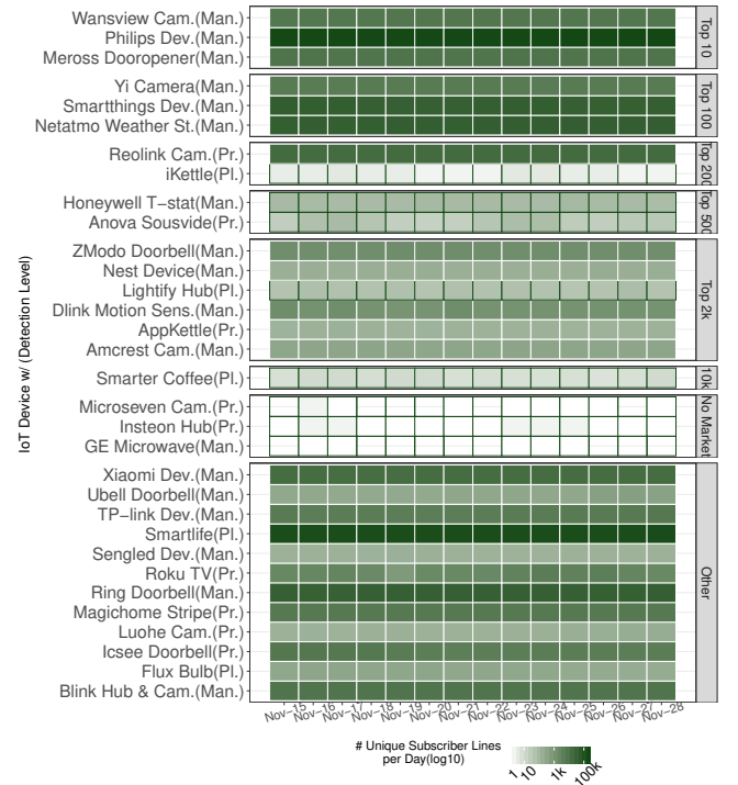
Figure 14: ISP: Drill down of IoT activity for 32 different IoT device types with their popularity in the ISPs country.
