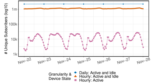
Figure 18: ISP: # Subscribers with active Alexa Enabled/hour.
