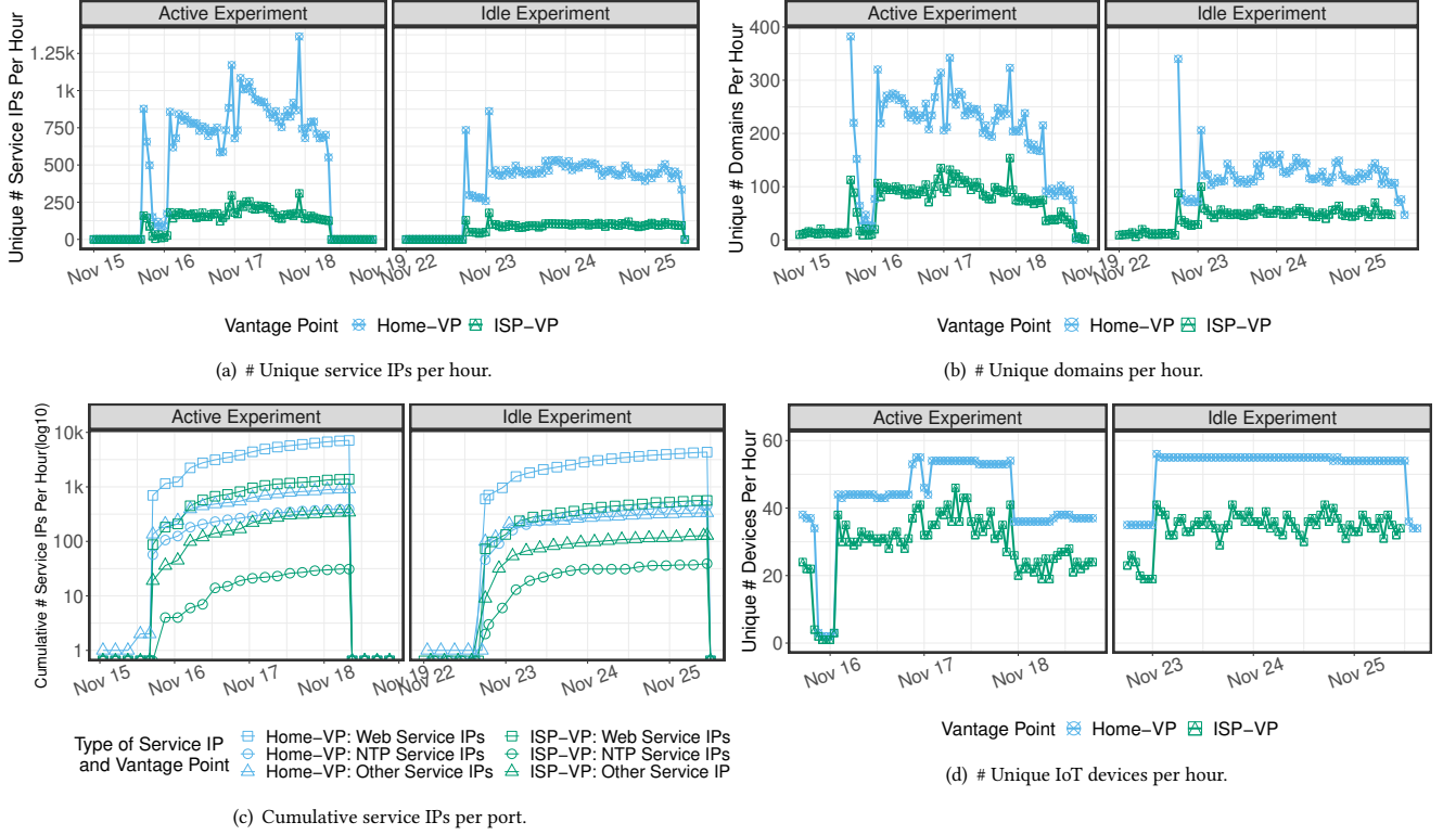
Figure 5: Home-VP vs. ISP-VP.
