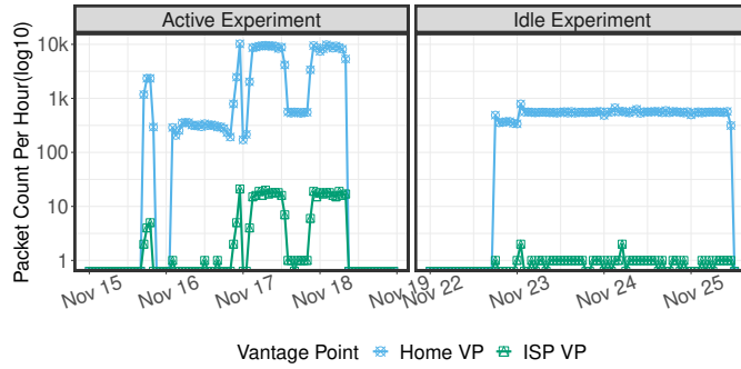
Figure 17: Home-VP/GT Household: Single Alexa Enabled device.
