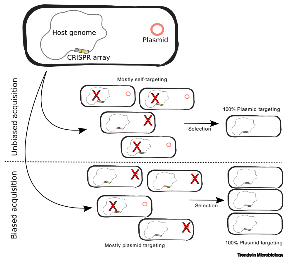
Figure 1. Observed Frequencies of Self-Targeting Spacers Can Lead to Underestimates of the Actual Rate of Autoimmunity. When acquisition is unbiased, strong selection against self-targeting spacers will purge them from the population. When acquisition is biased, self-targeting spacers will not be acquired in the first place. In both cases, the population will end up with very few self-targeting spacers. Thus, even CRISPR systems that lack a mechanism for self versus non-self recognition may appear to prefer non-self spacers on the basis of population-level immune diversity.
