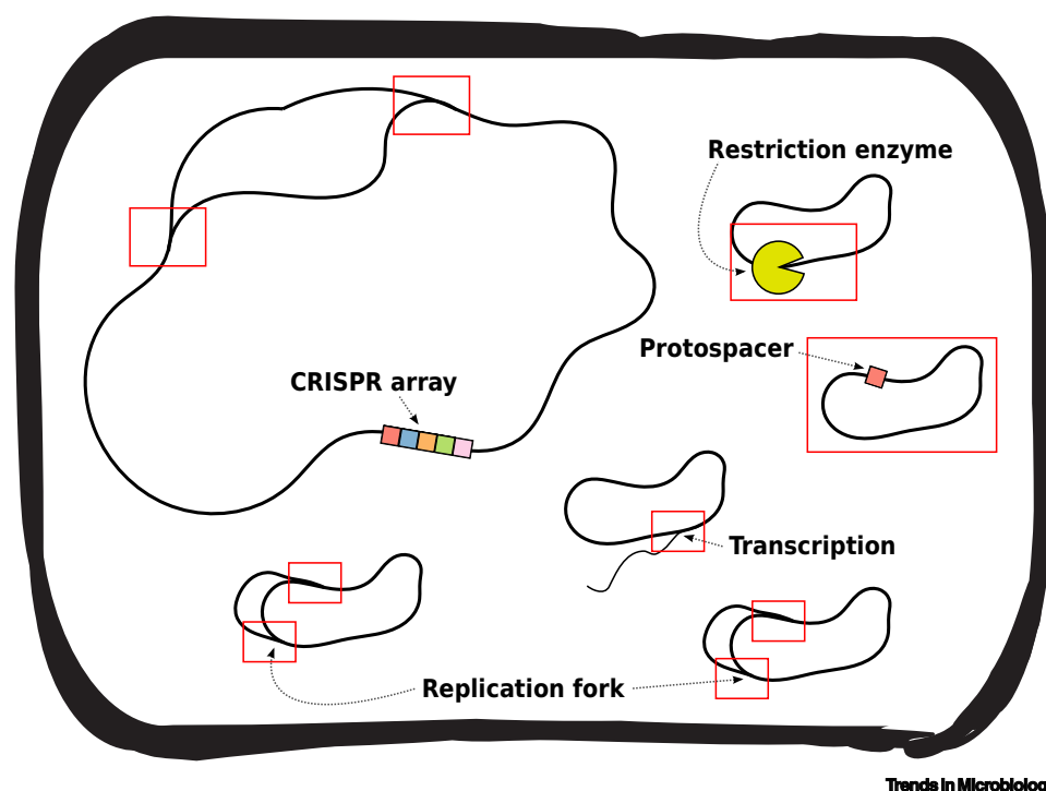
Figure 2. Multiple Mechanisms for Non-self Recognition May Rely on the Production of Excess Free DNA Ends by Mobile Genetic Elements. Drawn is a schematic of a host cell infected by multiple plasmids. Regions expected to experience a high rate of double-strand break formation are indicated by red rectangles.
