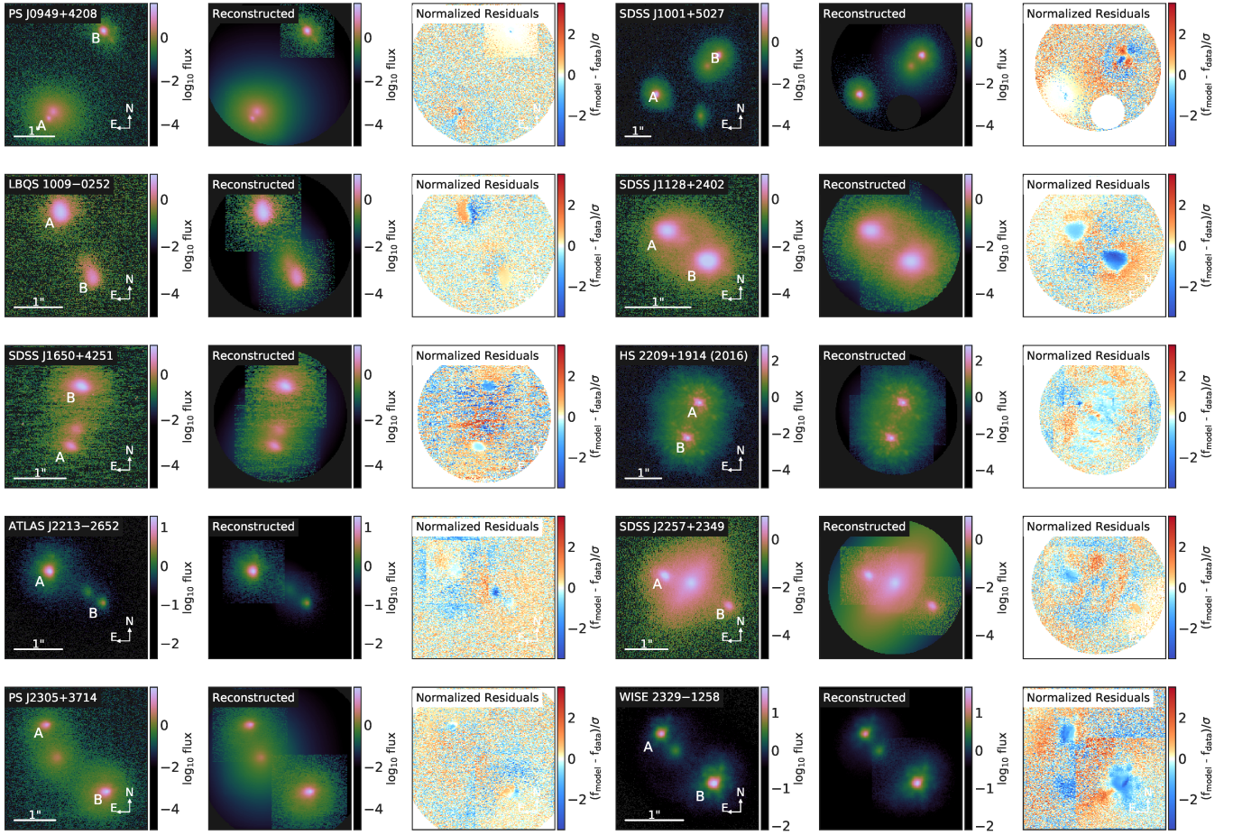
Figure 5. Continuation of Figure 4 for the last 10 doubles. We show only the 2016 image of HS2209+1914. However, both images from 2013 and 2016 were simultaneously used to model this system.
