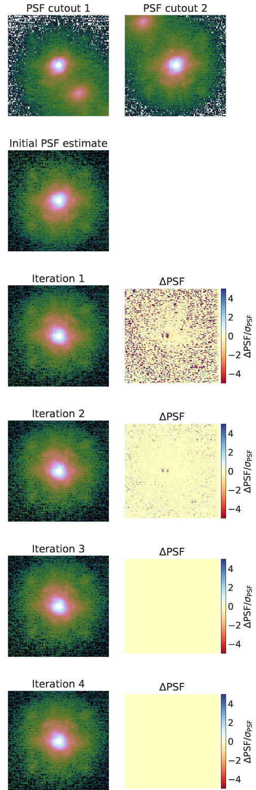
Figure 3. Estimation of the initial PSF and PSF reconstruction through an iterative algorithm. This examples is shown for the system PS J0140+4107. The top row shows two cutouts centered at the quasar images. The contamination in the cutouts are removed through a weighted sum of the two cutouts to obtain the initial PSF estimate in the second row. The third to last rows show the reconstructed PSF through an iterative procedure (first column) described in Section 3.3 and the difference between the current PSF iteration with the previous one (second column). The reconstructed PSF typically converges after 2–3 iterations.
