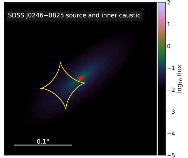
Figure 8. Reconstructed flux distribution of the quasar host galaxy in the SDSS J0246-0825 system. The red star marks the position of the central quasar. The yellow line traces the inner caustic.
