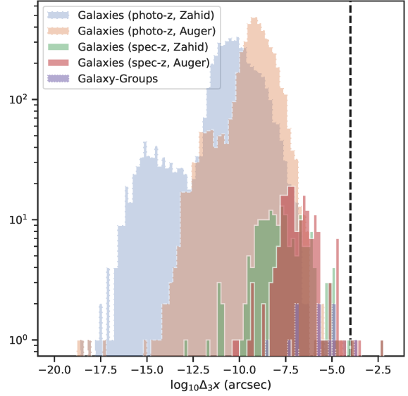
Figure 9. Flexion shift histograms for galaxies and galaxy groups in the environment of DES J0408–5354.
