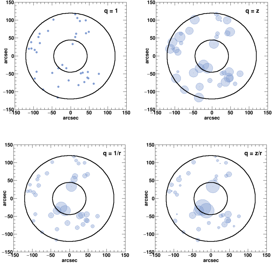
Figure 11. The relative weights of the galaxies around DES J0408–5354 for the four weighting schemes q = 1 , q_z = z_s \times z_i - z_i^2 , q_r = 1/r and q_{z/r} = (z_s \times z_i - z_i^2)/r . The galaxies satisfy i < 22.5 and are represented by circles with areas proportional to their weights. The black circles indicate the 120'' and 45'' apertures.
