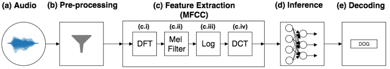
Figure 1: The steps that form the Automatic Speech Recognition pipeline. (a) The audio is recorded using a microphone. (b) It is preprocessed to remove any rudimentary noise or high frequencies using a low pass filter. (c) The audio is passed through a feature extraction function (in this case the MFCC function) that extracts the most important features of the audio sample. (d) The features are passed on to the model for inference, which outputs a non-human-readable string. (e) The string is decoded to produce a human-readable transcription.
