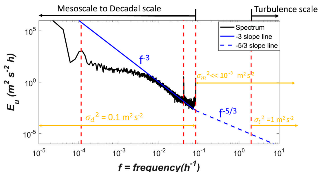
Figure 9. Energy spectrum of global average 6-hourly wind speed. The spectrum is extrapolated from 12 h to a turbulence scale (seconds) via Kolmogorov's f^{-5/3} power law ( f^{-5/3} , blue dashed line). The resolved spectrum has an exponent of -3 from multi-day to 12 h ( f^{-3} , blue solid line) consistent with an enstrophy cascade in a quasi-geostrophic flow. The dashed vertical lines (right to left) indicate frequencies corresponding to the following timescales: sub-hour ( =0.5 h), diurnal ( =12 h), daily ( =24 h), and annual ( =8760 h), respectively. The \sigma_d^2 , \sigma_m^2 , and \sigma_t^2 refer to the variance at large (mesoscale to decadal), intermediate (12 h to turbulence), and small (turbulence) scales, respectively.
