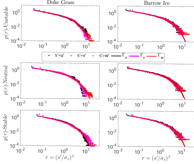
FIG. 2. The empirical distribution of r = (s'/\sigma_s)^2 for s'^2 = u'^2 , s'^2 = v'^2 , and s'^2 = w'^2 along with a fitted \gamma distribution for each velocity component. The \gamma fit was obtained using a maximum likelihood estimation.
