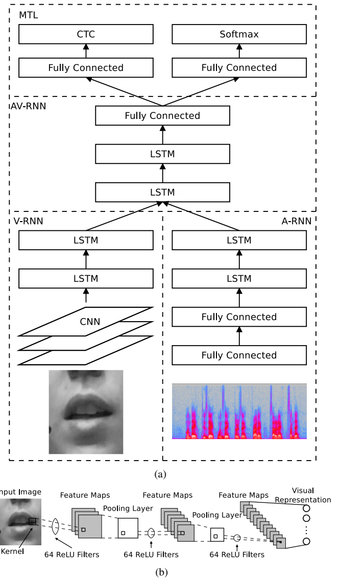
Fig. 2. (a) Diagram of the proposed end-to-end MTL framework, which consists of three sub-networks. The A-RNN sub-network processes raw audio input relying on FC and LSTM layers. The V-RNN sub-network processes raw video input relying on CNN and LSTM layers. The activation from the A-RNN and V-RNN sub-networks are concatenated and sent to the AV-RNN sub-network. The final high-level feature representation is used to solve two speech tasks: AV-ASR and AV-VAD. (b) Diagram of the CNN-based architecture used in the V-RNN sub-network.
