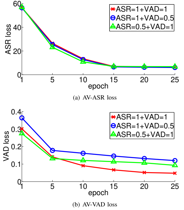
Fig. 4. Loss during training for the primary and secondary tasks. The figure shows that the ASR loss dominates the total loss, which explains the good performance of the proposed approach even when \alpha_{asr} \leq \alpha_{vad} .
