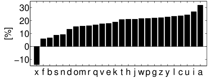
Fig. 5. Relative improvement in ASR performance for each character by considering facial features in addition to audio features (i.e., A-ASR versus AV-ASR systems). The figure reports the results on the test set under challenging condition in noisy environment.
