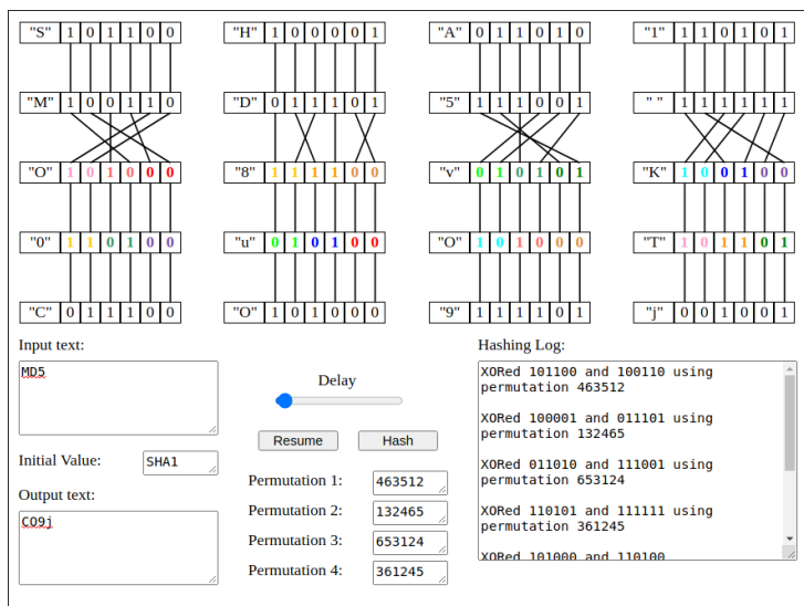
Figure 4: Hashing tool
