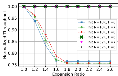
FIGURE A.4: Throughput of uni-regular topologies under expansion.
