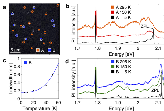
Figure 2. Spectral analysis of quantum emitters in thin-film w-AlN. (a) Quantum emitter density in a 25\ \mu\text{m} \times 25\ \mu\text{m} area (white scale bar: 5\ \mu\text{m} ). Two types of emitters with orthogonal polarization states are identified, labeled as “A” and “B”. (b) Temperature-dependent PL spectra of a representative type A quantum emitter (black, 5 K; red, 150 K; orange, 295 K), with the zero-phonon line (ZPL) indicated for the 5 K spectrum. (c) Temperature dependence of the type B quantum emitter’s ZPL line width. (d) Temperature-dependent PL spectra of a representative type B quantum emitter (black, 5 K; green, 150 K; blue, 295 K), with the ZPL indicated for the 5 K spectrum.
