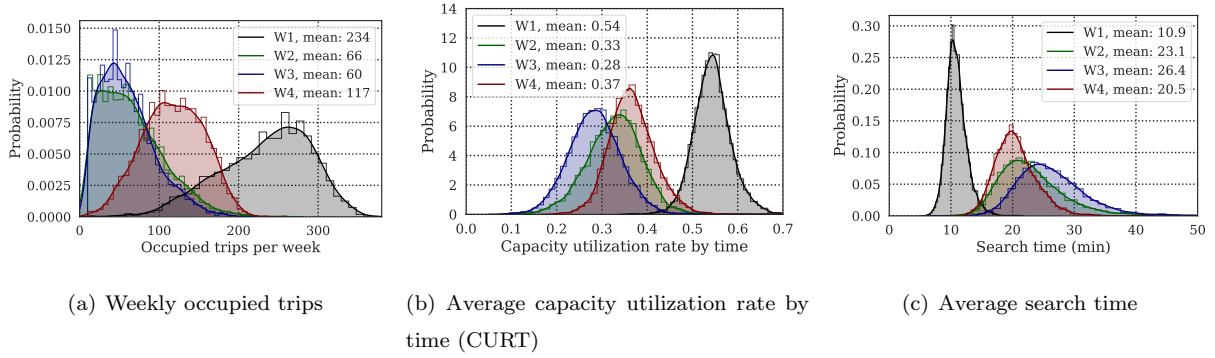
Figure 12: Productivity metrics of the 5,021 taxis in the four weeks. (The mean value for each week is reported in each plot.)
