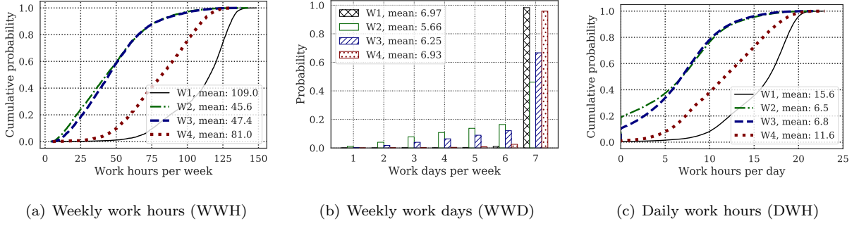
Figure 9: Work schedules of the selected 5,021 taxis in the four weeks. (The mean value for each week is reported in each plot.)
