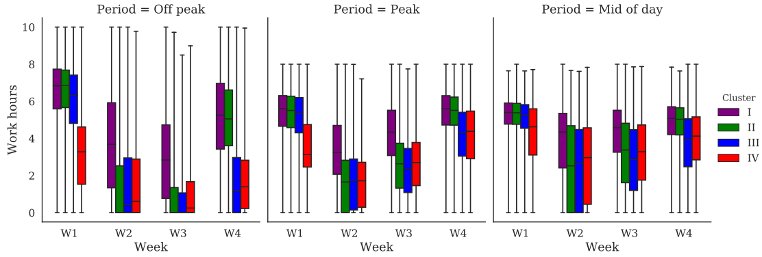
Figure 16: Clustered box plots for daily work hours (DWH) by periods.
