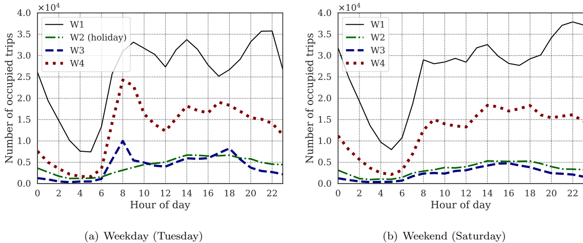
Figure 4: Number of hourly occupied taxi trips in the four weeks ( W_i , i = 1, 2, 3, 4 refers to Week i ).
