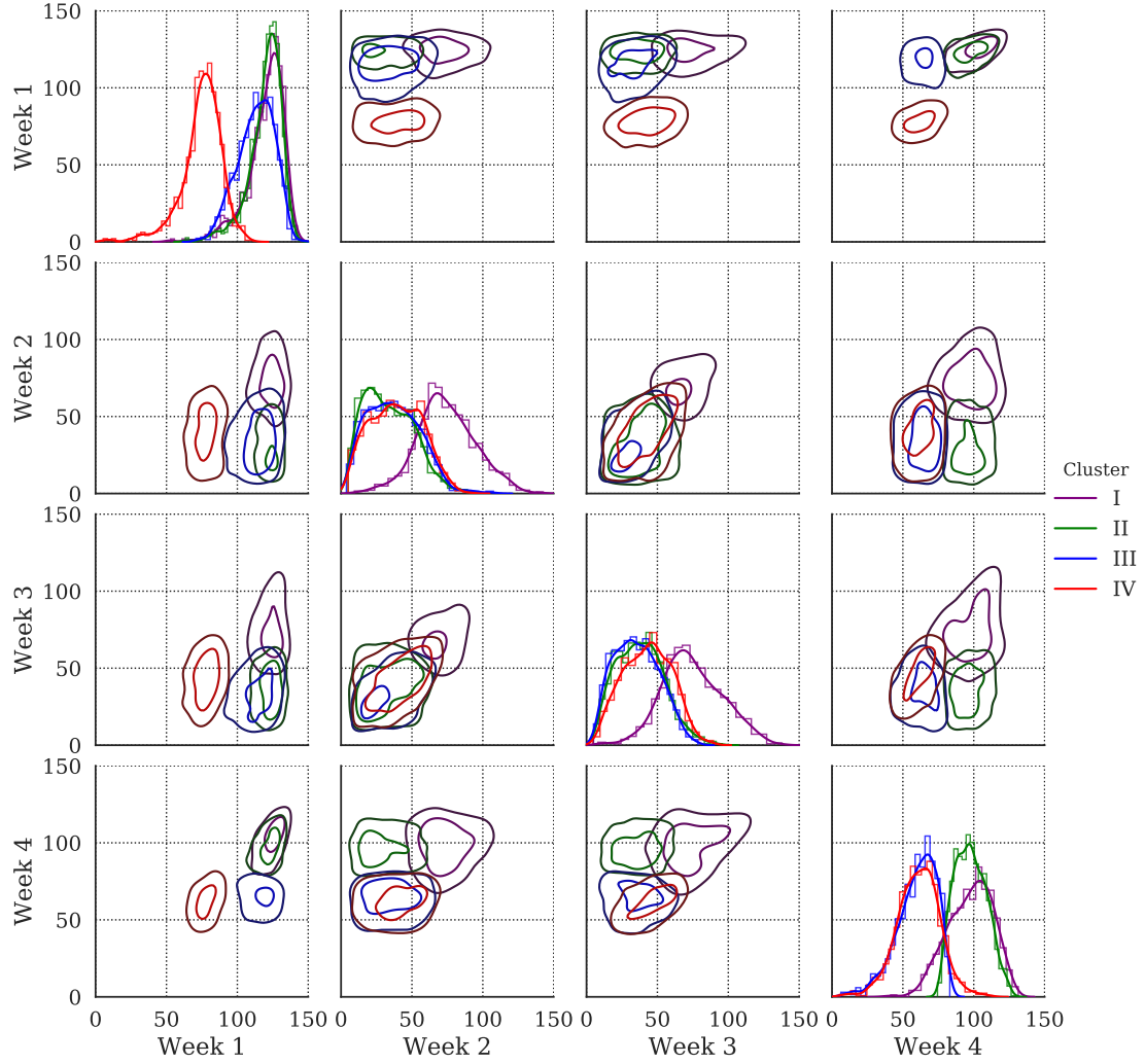
Figure 14: Clustered two-dimensional analysis of taxi weekly work hours. In each plot, both x and y axes represent WWH in one of the four weeks. The week number corresponding to each plot's axes can be read from the row (on the left) and column (at the bottom) indexes. Off-diagonal subplots are bivariate kernel density functions of WWH corresponding to the two different weeks on its axes, while diagonal plots show the PDFs of WWH in each week.
