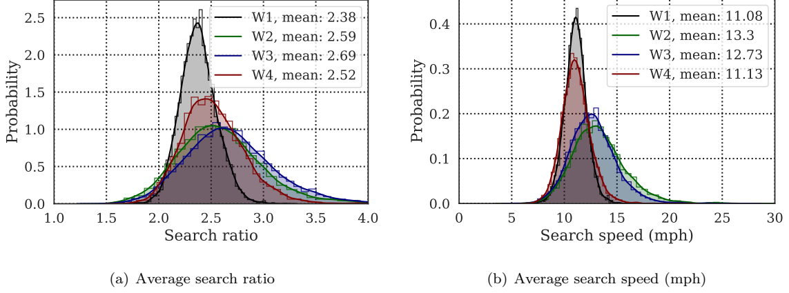
Figure 13: Search behaviors of the 5,021 taxis in the four weeks. (The mean value for each week is reported in each plot.)
