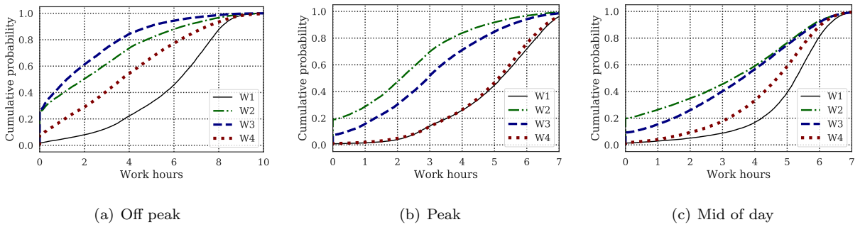
Figure 10: CDF of daily work hours (DWH) in different periods of day.
