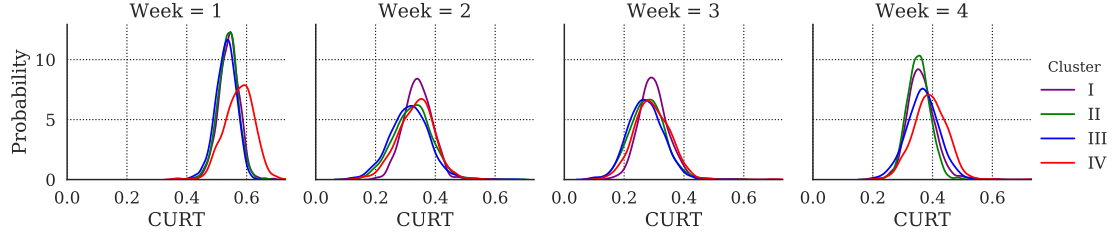
Figure 15: Clustered PDF of average capacity utilization rate by time (CURT).
