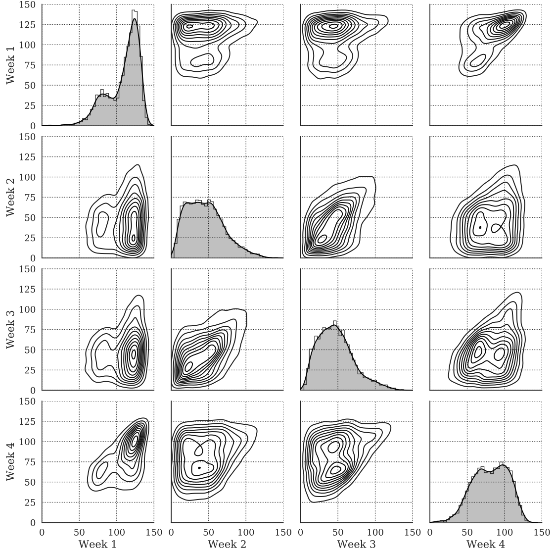
Figure 11: Two-dimensional analysis of taxi weekly work hours (WWH). In each plot, both x and y axes represent WWH in one of the four weeks. The week number corresponding to each plot's axes can be read from the row (on the left) and column (at the bottom) indexes. Off-diagonal subplots are bivariate kernel density functions of WWH corresponding to the two different weeks on its axes, while diagonal plots show the PDFs of WWH in each week.
