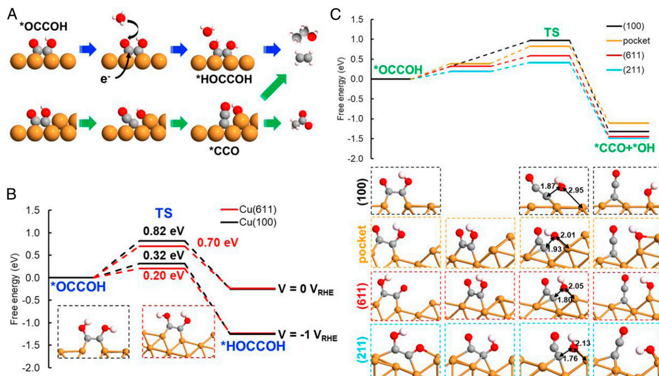
Fig. 4. Proposed reaction mechanism and the reaction energies on different Cu surfaces. (A) Proposed reaction mechanism for electroreduction of CO to C 2 + products. The blue path produces ethanol and ethylene, while the green path can also generate acetic acid. (B and C) Reaction free energies and barriers (B) to form *HOCCOH through PCET at 0 V RHE and -1 V RHE and (C) to dissociate *OCCOH to *CCO and *OH on Cu(100) in black, Cu pocket-shape in orange, Cu(611) in red, and Cu(211) in blue. Insets show the system geometries. Orange, red, gray, and white spheres represent Cu, O, C, and H, respectively. Numbers in Insets represent distance in angstroms. The left figure in the boxes in C represents the most stable *OCCOH geometry, while to the immediate right the adsorbate is oriented toward the edge prior to OCC-OH bond dissociation (e.g., the overall barrier is always referenced to the adsorbate on the flat terrace in its most stable configuration).
