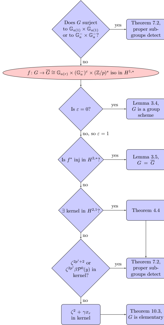
FIGURE 1. This flowchart for Theorem 1.2 may help in reading Sections 10 and 11.
