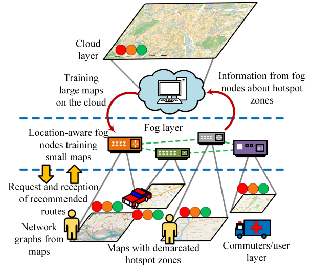
Figure 2: Network architecture for the S-Nav system.
