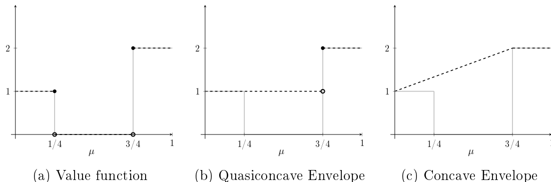
Figure 1: The simple think-tank example. The dashed lines represent the highest value the think tank can obtain from no information (left), cheap talk (center), and commitment (right).
