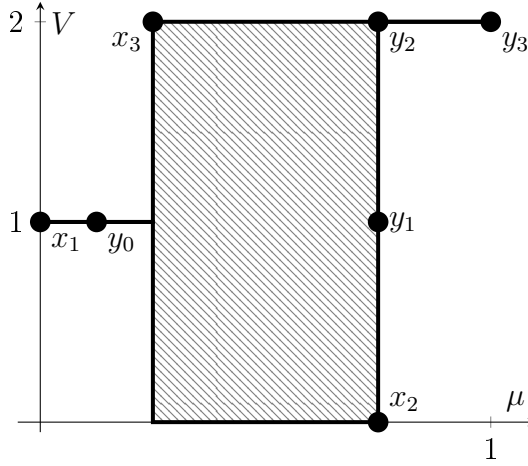
Figure 3: S’s value correspondence in an example where R strictly benefits from long cheap talk.
