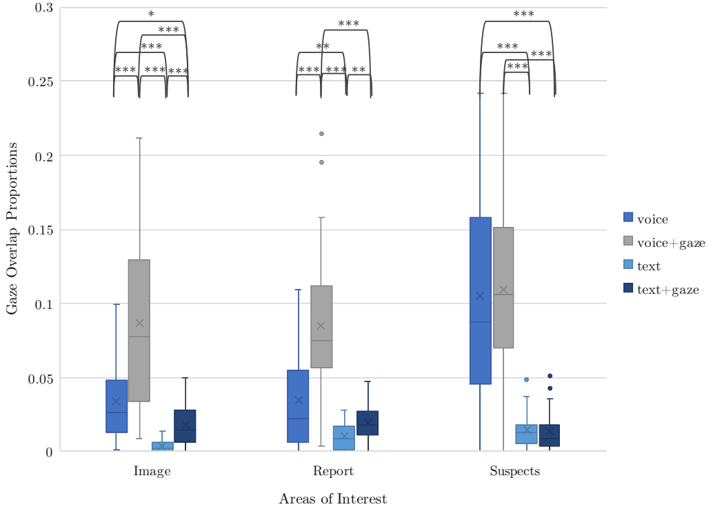
Fig. 4. The normalized gaze overlap proportions for the three AOIs: image, report, and suspects, across each of the four media. Statistically significant differences in scores are indicated for pairwise comparisons (* for p < .05 , ** for p < .01 , and *** for p < .001 ). Participants looked at the same AOIs for longer during voice-based communication. Shared gaze led to increases in gaze overlap both for voice- and text-based communication.
