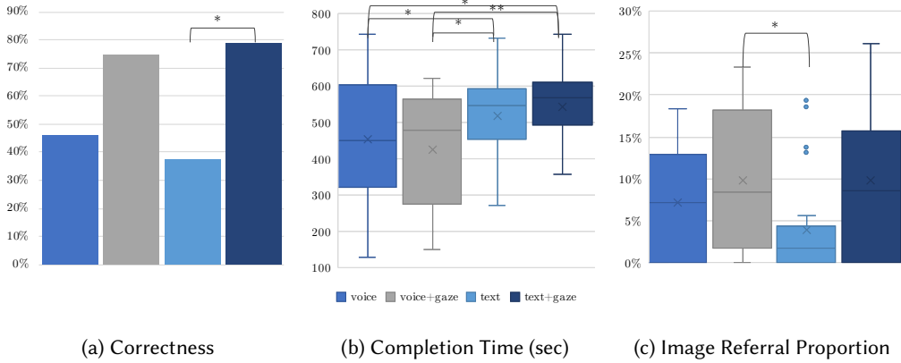
Fig. 2. Correctness (a), completion time (sec) (b), and image referral proportion (c) across the four conditions. Statistically significant differences are indicated for pairwise comparisons (* for p < .05 , ** for p < .01 , and *** for p < .001 ). Shared gaze leads to more correct answers and higher referrals on the shared image for both voice- and text-based communication. Completion time is shorter for voice and longer for text-based communication, with shared gaze having the opposite effect on the two.
