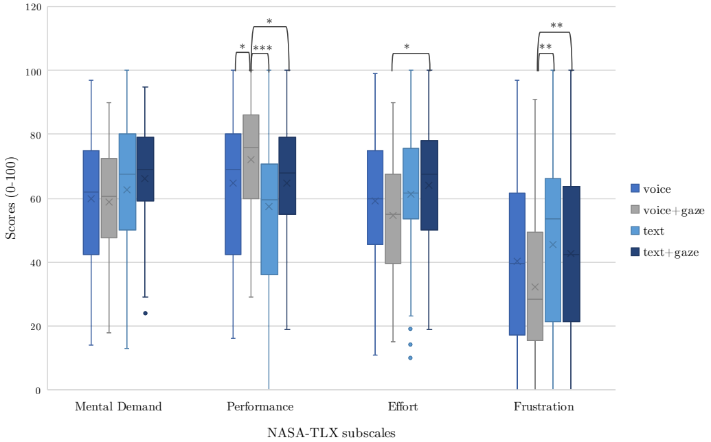
Fig. 5. The four subjective subscales of the NASA-TLX questionnaire that were asked at the end of each task to capture the cognitive workload. Statistically significant differences in scores are indicated for pairwise comparisons (* for p < .05 , ** for p < .01 , and *** for p < .001 ). Voice leads to less cognitive workload than text communication. Shared gaze further improves voice while having the opposite effect on text.
