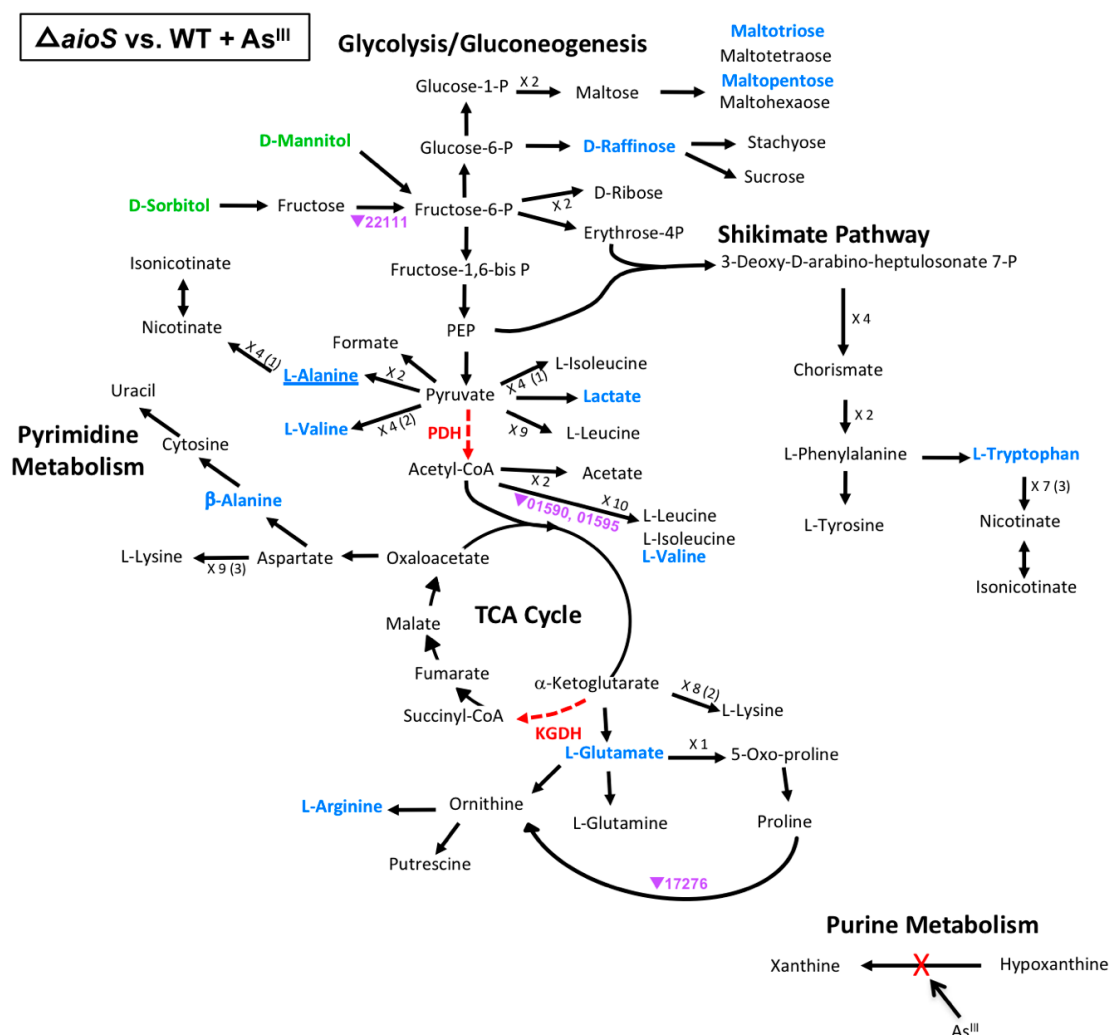
Figure 4. Model of carbon metabolism in the \Delta aios mutant vs WT during As III exposure, with mannitol being the initial substrate. Reaction steps were derived from KEGG pathway maps using the most parsimonious routes of metabolite formation, noting that not all enzyme reaction steps are depicted in the model. When multiple intermediates are involved between illustrated metabolites, the number of reactions is shown; i.e., \times 3 , with the number of intermediates identified shown in parentheses. Green text denotes metabolites increased in abundance; blue text denotes metabolites decreased in abundance. Red dashed vector arrows indicate reactions suggested to be inhibited by As III . Transcripts are denoted by AT5A identification number (purple text), with a triangle indication increased expression ( \blacktriangle ) or decreased expression ( \blacktriangleleft ). Underlined text indicates metabolites or transcripts for which the change in abundance when compared to the WT was the same with or without As III .
