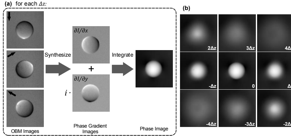
Fig. 2. (a) Procedure for reconstructing qualitative images from raw 3-angle OBM images. (b) Reconstructed 9-depth qualitative phase image of a single 45 μm polystyrene bead. \Delta z = 29.5 \mu\text{m} .
