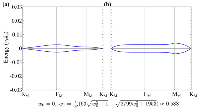
FIG. 14. Comparison between (a) the active bands of the BM model at the w_0 = 0 , w_1 \approx 0.588 point and (b) the bands of the two-band first order approximation to H_{\text{Approx1}}(\mathbf{k}) in Eq. (33). Notice that the bandwidth at the \Gamma_M point is virtually identical, that the bands are flat, and that they close gap at the K_M point.
