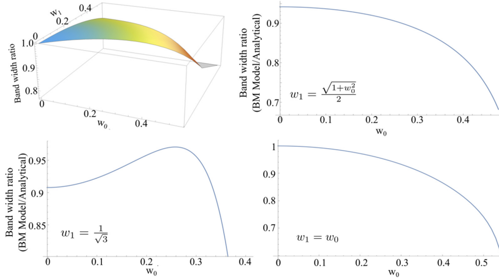
FIG. 11. Plots of the ratio of the bandwidth of the active bands for the large number of shells to the analytic bandwidth \Delta in Eq. (56), for different values of w_0, w_1 , including the two magic manifolds. In the regime of validity of our approximations, we can see that this ratio is substantially above 90%.
