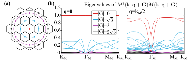
FIG. 5. The magnitude of the form factor (overlap matrix) M^{(\eta=+)}(\mathbf{k}, \mathbf{q} + \mathbf{G}) , calculated for w_0 = 0.4745 and w_1 = 0.5931 . (a) The colored dots are the \mathbf{G} vectors we consider in M^{(\eta=+)}(\mathbf{k}, \mathbf{q} + \mathbf{G}) . Different colors represent different length of \mathbf{G} . (b) The eigenvalues of M^{(\eta=+)}(\mathbf{k}, \mathbf{q} + \mathbf{G})M^{(\eta=+)}(\mathbf{k}, \mathbf{q} + \mathbf{G}) as functions of \mathbf{k} . In the left and right panels we choose \mathbf{q} = 0 and \mathbf{q} = \frac{1}{2}\mathbf{k}_M , respectively, where \mathbf{k}_M is the M_M momentum in the moiré BZ.
