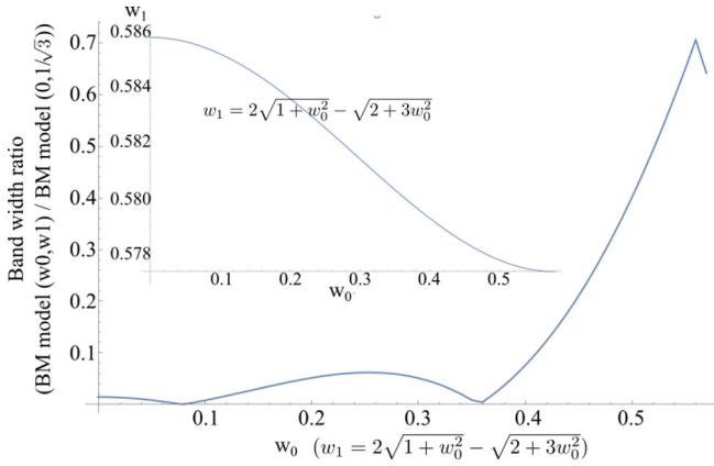
FIG. 12. \Gamma_M point bandwidth of the active bands (large number of shells) on the manifold \Delta(w_0, w_1) = 0 ( w_1 = 2\sqrt{1 + w_0^2} - \sqrt{2 + 3w_0^2} ) of zero analytic bandwidth [Eq. (56)] divided by the bandwidth of the active bands in the chiral limit [ (w_0, w_1) = (0, \frac{1}{\sqrt{3}}) ]. Note that this number is extremely small away from w_0 = w_1 = \frac{1}{\sqrt{3}} , showing that our analytic manifold of smallest bandwidth [ \Delta(w_0, w_1) = 0 ] also exhibits small bandwidth in the large cell number. Inset: The curve w_1 = 2\sqrt{1 + w_0^2} - \sqrt{2 + 3w_0^2} for which \Delta(w_0, w_1) = 0 for 0 \leq w_0 \leq \frac{1}{\sqrt{3}} . Note that w_1 changes extremely little 1% (stays within 1% of \frac{1}{\sqrt{3}} ) during the entire sweeping of w_0 .
