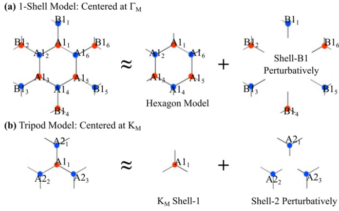
FIG. 8. The two types of approximate models used for analytics. (a) The one-shell (A1, B1) model which we have theoretically argued and numerically substantiated to represent a good approximation for values w_0, w_1 \leq 1/\sqrt{3} . Analytically we will first solve it by perturbation theory around the hexagon model, which involves only the A1 sites. The shell B1 will be added perturbatively to obtain H_{\text{Approx1}}(\mathbf{k}) in Eq. (33). (A second way to solve for this Hamiltonian will be presented later.) (b) The tripod model, which involves the two shells A1 (also known as the K_M point) and A2. Due to the same considerations as for the \Gamma_M -centered model, this should be a good approximation for the infinite shell model for w_0, w_1 \leq 1/\sqrt{3} . This is the same model as solved by Bistritzer and MacDonald [1]. We find that the magic angle at which the Dirac velocity vanishes at the K_M point is given by w_1 = 1/\sqrt{3} , \forall w_0 .
