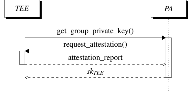
Figure 2: CACTI provisioning protocol. The interaction between the Provisioning Authority (PA) and the client’s TEE takes place over a secure connection, using the client to pass the encrypted messages. After verifying the attestation report (and any other required information), the PA provisions the TEE with a group private key ( sk_{TEE} ).
