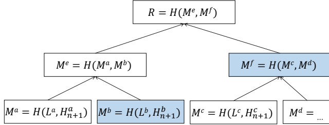
Figure 5: Merkle Hash Tree over lists a...d . Each leaf is a hash of the list information L^i (list name and public key) and the most recent hash of the list's hash chain H_{n+1}^i . H() is a cryptographic hash function, R is the root of the MHT, and the nodes in blue illustrate the inclusion proof path for list b .
