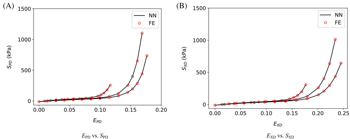
FIGURE 10 Verification of the FE implementation with the NN model for three planar biaxial test protocols: E_{PD} : E_{XD} = 1 : 1, 0.17 : 0.23, 1 : 3
