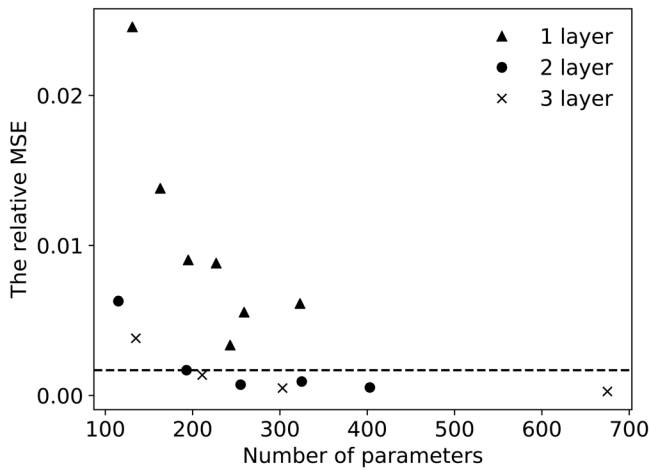
FIGURE 3 The training error of NNs with different numbers of layers and neurons
