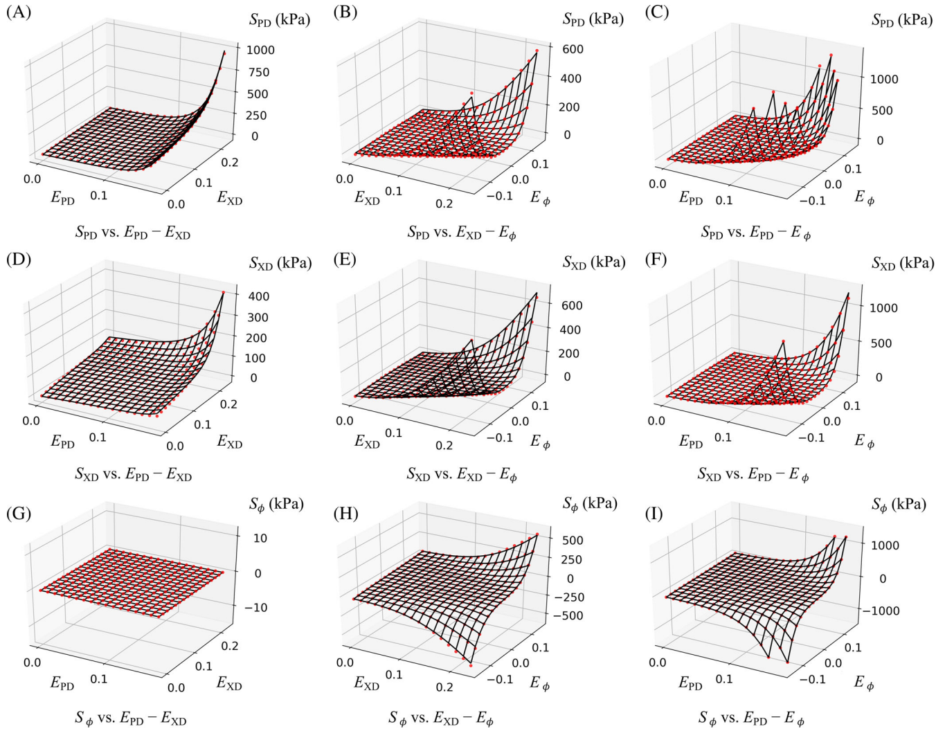
FIGURE 5 Graphical depiction of the strain ranges used to train the NN model. Also shown are the validation results for the final NN model for \sigma = 25.48^\circ
