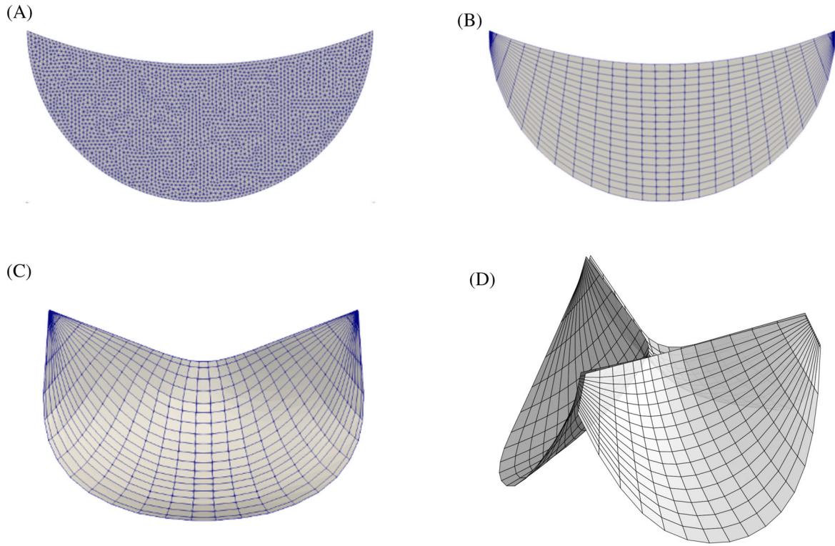
FIGURE 7 The 2D triangular mesh (A) is first fit by a 2D NURBS mesh (B) to interpolate fiber ODFs on the NURBS mesh. Then the fiber ODFs at a point \mathbf{X}_0 on the 2D NURBS mesh can be mapped to the corresponding point \mathbf{X} on the 3D leaflet geometry (C). The NURBS mesh (D) for simulations consists of three identical 3D leaflet geometries with cropped corner to improve the mesh quality
