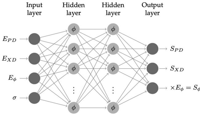
FIGURE 6 A schematic of the final fully connected NN model for planar mechanical behavior of native and replacement heart valve leaflet soft tissues. The input nodes consist of the strain tensor components and the \Gamma standard deviation. The output is the three stress tensor components. Note that the shear stress term is post-multiplied with the shear strain, resulting in that zero shear strain gives zero shear stress as fitting constraint (see text for details)
