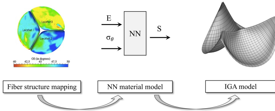
FIGURE 1 A schematic of the computational pipeline for integrated IGA-based model utilizing the NN material model and tensor-mapped fiber structure
