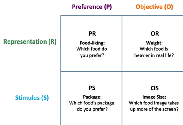
Fig. 1 Experimental setup. Past research has made a distinction between value-based decisions and perceptual decisions. However, these two types of decisions typically vary along multiple dimensions: whether the decision is based on a mental representation of a stimulus or on the stimulus itself, and whether the decision is based on subjective preference or objective criteria
